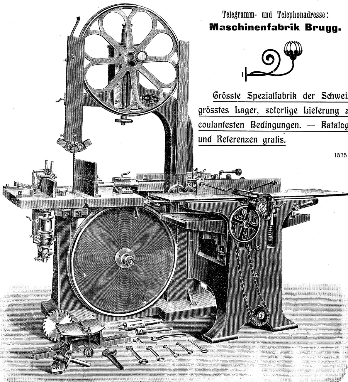
Universalmaschine No. 3.
