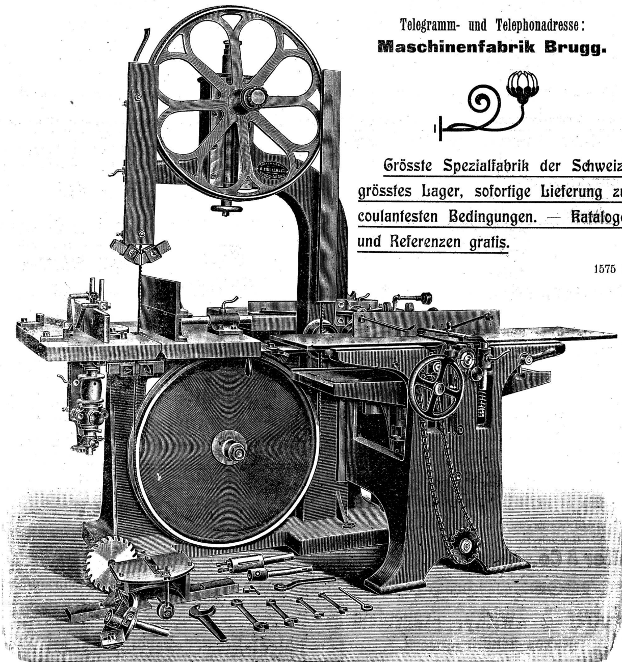
Universalmaschine No. 3.
