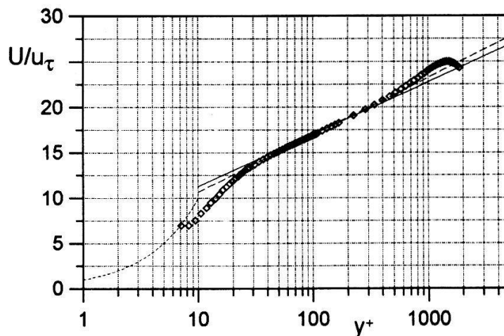
Fig. 1: Mean stream velocity U normalized with the friction velocity u_\tau as a function of the normalized wall distance y^+ at U_{cl} = 14 \frac{m}{s} . \diamond : experimental data, \cdots : viscose sublayer ( u^+ = y^+ ), - : logarithmic law (Eq. 1), - - : fit to the present logarithmic law ( u^+ = 2.73 \ln y^+ + 4.37 )
