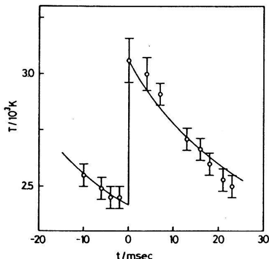
Fig.1 Typical cooling rate to 400 \mu m Ta droplets
