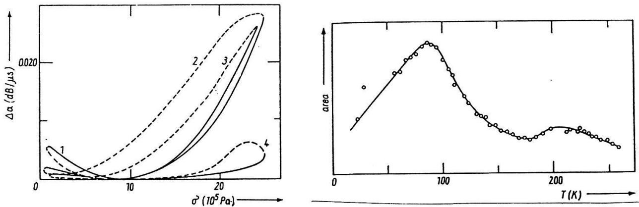
Fig. 4 (a). The BR signatures measured at different temperatures [(4) 39K, (2) 85K, (3) 217K]. The frequency of the applied stress is 0.02 Hz and the frequency of the ultrasounds is 8.5 MHz. (b) The surface of the BR signatures as a function of the measurement temperature.
