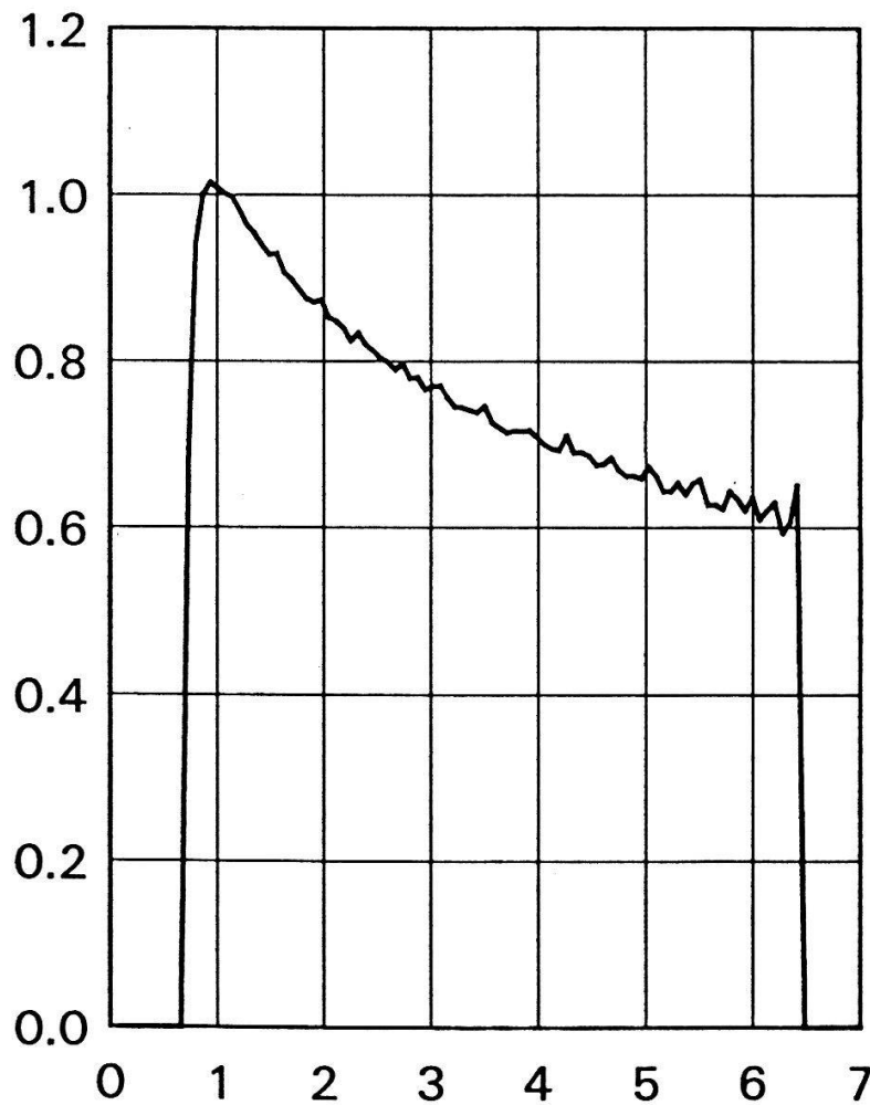
Figure 3: The distribution f(\alpha) of Hölder exponents \alpha for the curve \beta(\zeta) ; the upper limit of \alpha = 6.5 is due to the quadruple accuracy of the calculations which sets every number smaller than 10^{-33} equal to 0.
