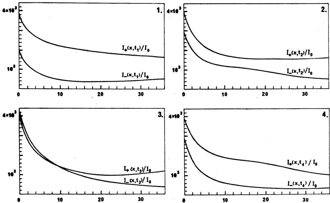
Fig. 2 Instantaneous spatial distributions of the normalized flux intensities I_{\pm}(x, t)/I_0 for times shown in Fig.1
