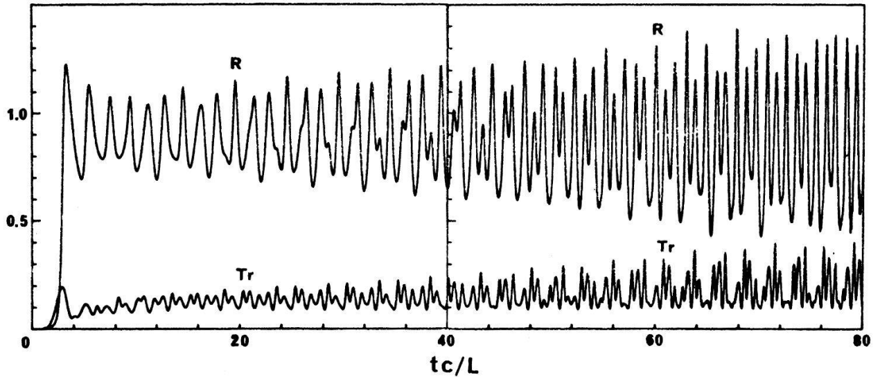
Fig. 4 Time dependent R and Tr for the multiple backscattering model governed by Eqs. (8)-(9)
