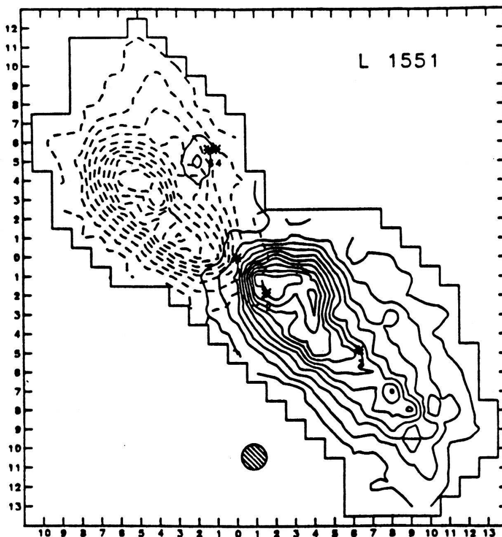
Figure 2 : bipolar morphology of the redshifted (broken lines) and the blueshifted (solid lines) molecular gas near L1551 (center of the map). From (2).
