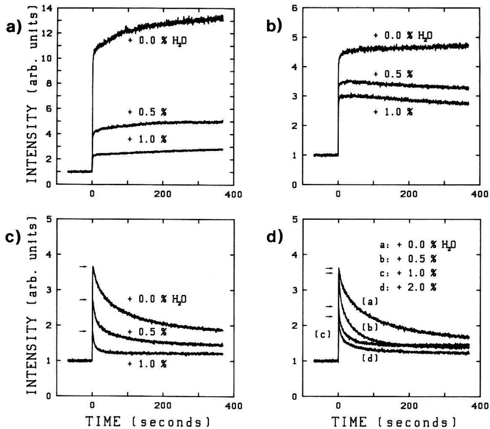
Fig. 3. Evanescent-wave-induced luminescence intensity versus time during solidification of DCM dye doped DMSO film for different film thicknesses a) d_0 = 10 \mu\text{m} , b) d_0 = 3.5 \mu\text{m} , c) d_0 = 1.2 \mu\text{m} , and d) d_0 = 0.6 \mu\text{m} . Parameter is the water content of the DMSO.
