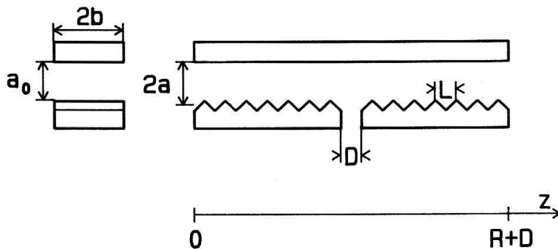
Fig. 1 Schematic of waveguide
