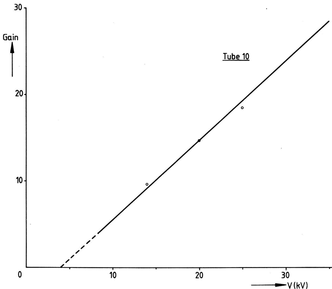
Figure 6. Gain as a function of accelerating voltage.
