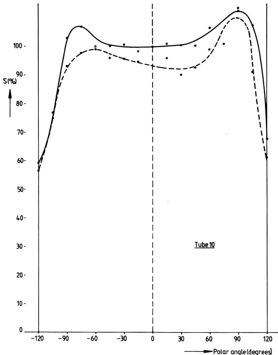
Figure 5. Relative sensitivity as a function of polar angle, for two azimuthal angles.
