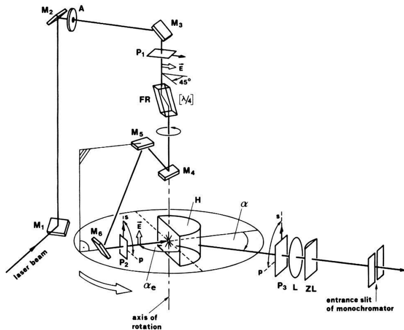
Fig. 2. Schematic of experimental set-up: H, hemicylindrical prism (cf. Fig. 1a); M_j , mirrors; P_j , polarizers; FR, \lambda/4 -Fresnel-rhomb; the optics (polarizer P_3 , lens L, cylindrical lens ZL) before the monochromator defines the emission angle \alpha and the polarization (s), (p).
