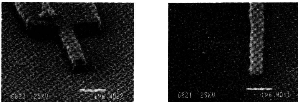
Fig. 1 SEM pictures of a contact strip. Its width is 0.5\ \mu\text{m} .
