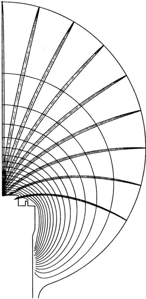
Figure 2. Electron trajectories showing 100% collection efficiency up to 90° polar angle.
