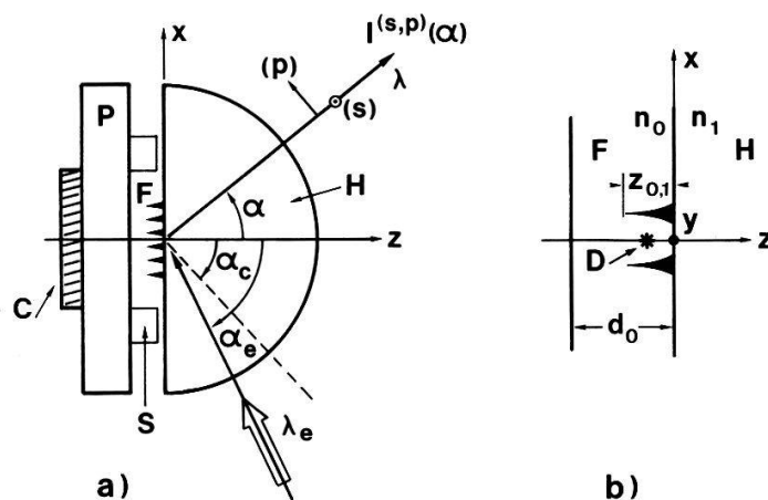
Fig. 1. a) Schematic of experimental set-up: H, hemicylindrical high index prism ( n_1=1.89 ); F, solidifying film of refractive index n_0 (DMSO doped with DCM laser dye); P, glass plate; C, Peltier cooler; S, spacers ( d_0 = 0.6, 1.2, 3.5 , and 10 \mu\text{m} ); \alpha_e , angle of incidence of exciting laser beam of wavelength \lambda_e ; \alpha_c = \arcsin(n_0/n_1) ; \alpha , angle of emission of luminescent light of wavelength \lambda ; (s), (p), polarizations; b) D, luminescent molecule in film F; z_{0,1} , penetration depth of evanescent wave.
