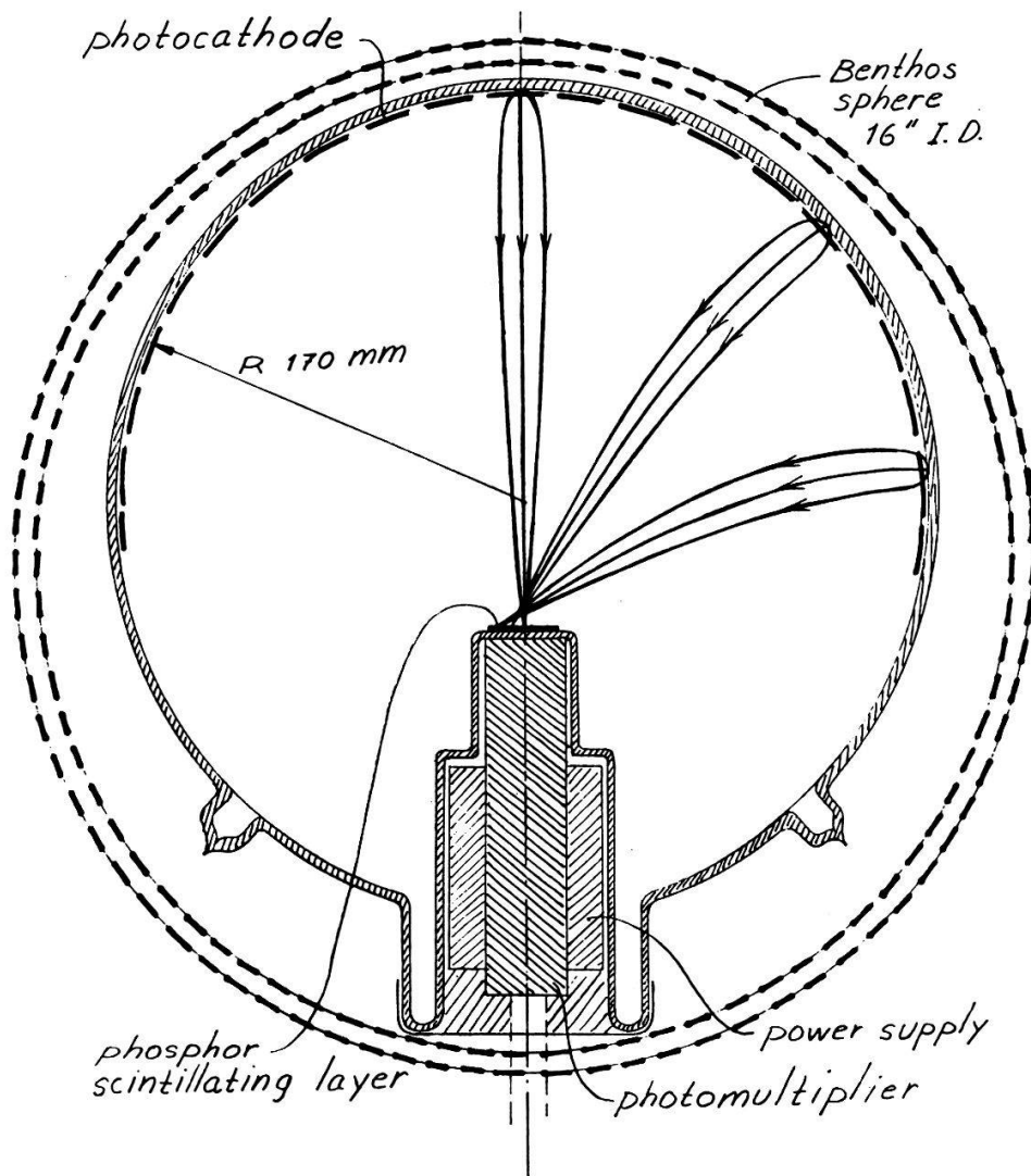
Figure 1. Design, schematically.
