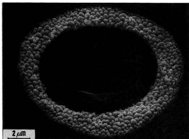
Fig. 3: Scanning electron microscope (SEM) picture of an annular Ga deposit formed in pyrolytic LCVD. The experimental conditions are the same as Fig. 1b. The deposit is quite irregular and consists mainly of quite large and amorphous particles.
