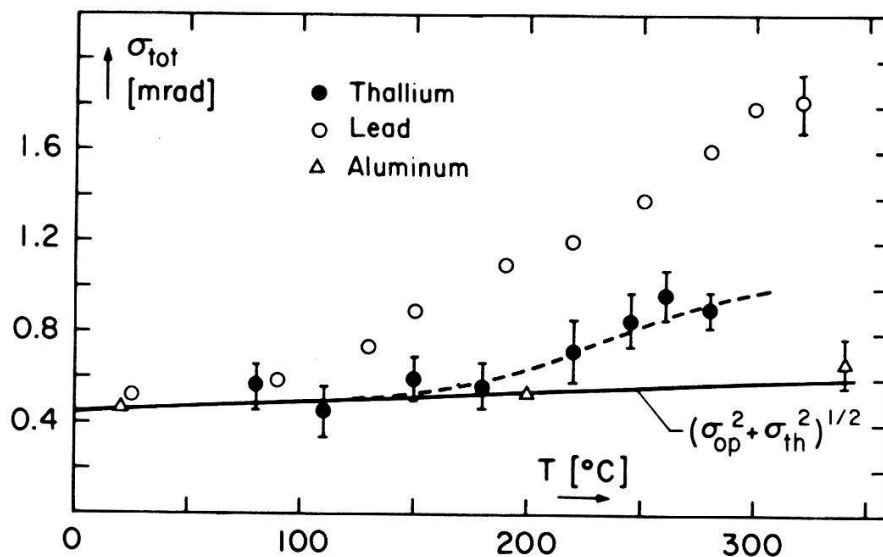
Fig. 1 Temperature dependence of \sigma_{tot} for Al, Tl and Pb. Dotted curve calculated from (2).
