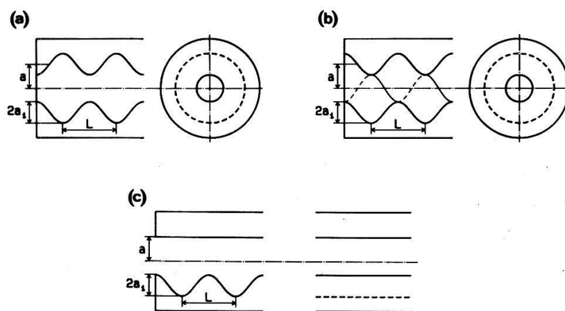
Fig. 1 Three types of corrugated waveguides
