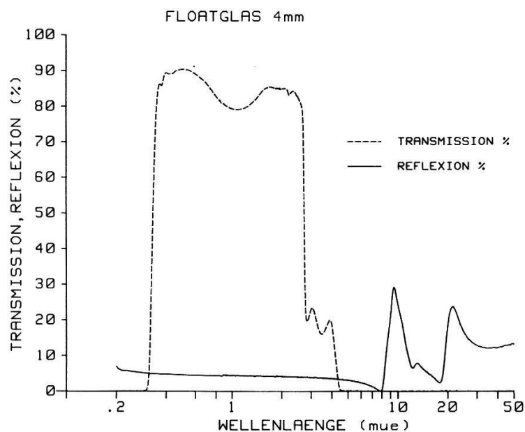
Fig. 1 Spectral transmission and reflection of "float" glass.
