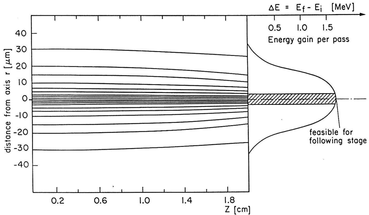
Fig. 1 Electron trajectories and energy gain in a linear periodic cylindric waveguide for axially injected electrons.
