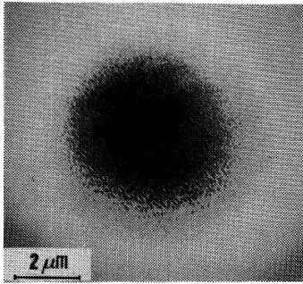
Fig. 4a: TEM picture of photodeposited Ga. The experimental conditions are: trimethylgallium pressure is 10 torr, the wavelength is 257.2 nm, exposure time is 60 s, the power density is 500 \text{ W cm}^{-2} . This deposit is significantly more homogeneous than the pyrolytically deposited Ga of Fig. 1a.
