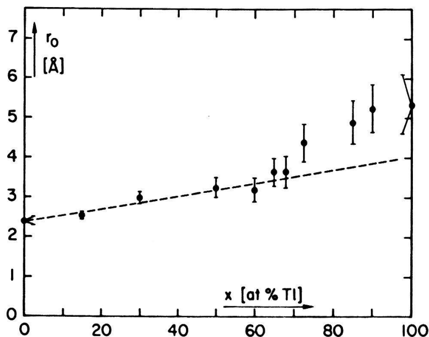
Fig. 2 Localization length r_0 versus Tl-concentration x in \text{Tl}_x\text{Pb}_{1-x} .
