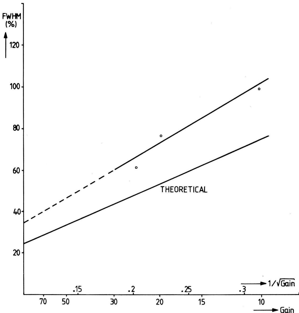
Figure 8. FWHM resolution as a function of gain. Theoretical curve and measurements.
