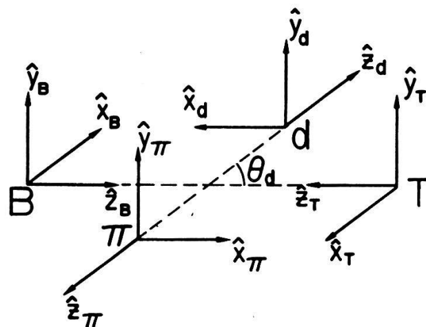
Fig.1: helicity reference frame used in this work.
