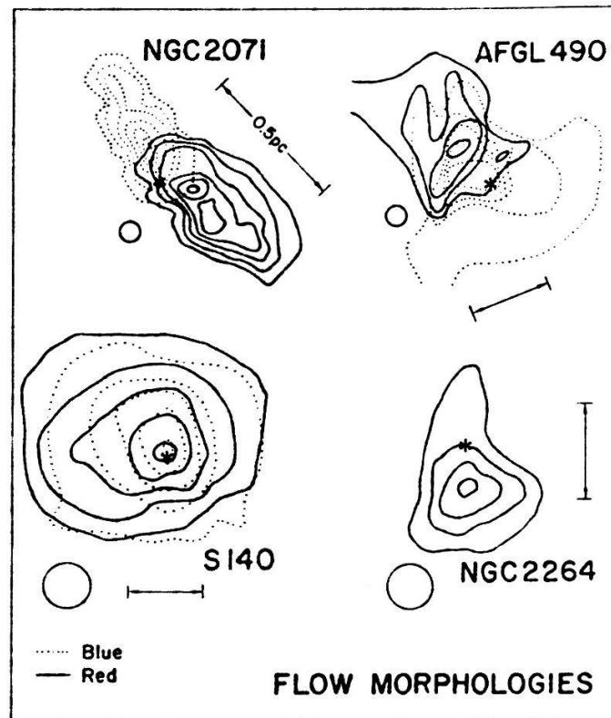
Figure 3 : flow morphologies : bipolar, multipolar, isotropic, unipolar. From (1).
