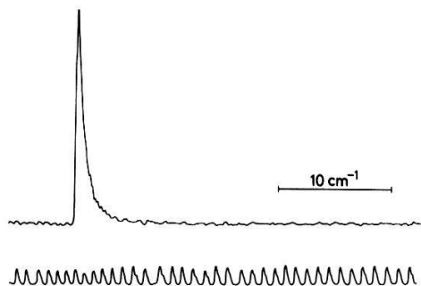
Fig. 3C : Measured rotational temperature of I_2(X) in the free jet. T_{\text{rot}} \approx 3 K.
