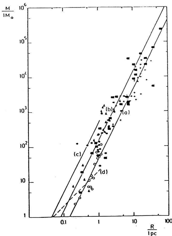
Fig.1: The mass-radius relation for molecular clouds.
