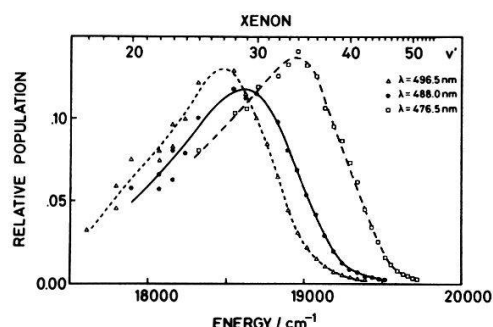
Fig. 1B : The relative vibrational populations of the B state of free \text{I}_2 after photodissociating \text{I}_2\text{Xe} at 496.5 nm ( \Delta ), 488 nm ( \bullet ), and 476.5 nm ( \square ). Conditions as in 1A. Energy is relative to X^1\Sigma^+ ( v'' = J'' = 0 ).
