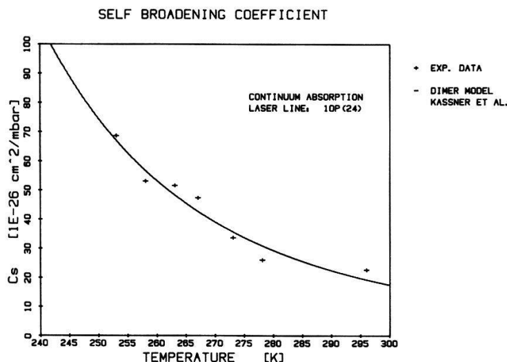
Fig. 2 Temperature dependence of the water-pressure quadratic component of the continuum absorption at the 10P(24) \text{CO}_2 -laser transition. The solid line represents the best fit based on the dimer model.
