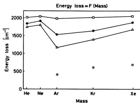
Fig. 2 : The mean energy lost by the cage effect in the photodissociation of \text{I}_2\text{M} for \text{M}=\text{He}, \text{Ne}, \text{Ar}, \text{Kr}, \text{Xe} at 496.5 nm ( \Delta ), 488 nm ( \bullet ), and 476.5 nm ( \square ). ( \circ ) are results of trajectory calculations (ref. 7).
