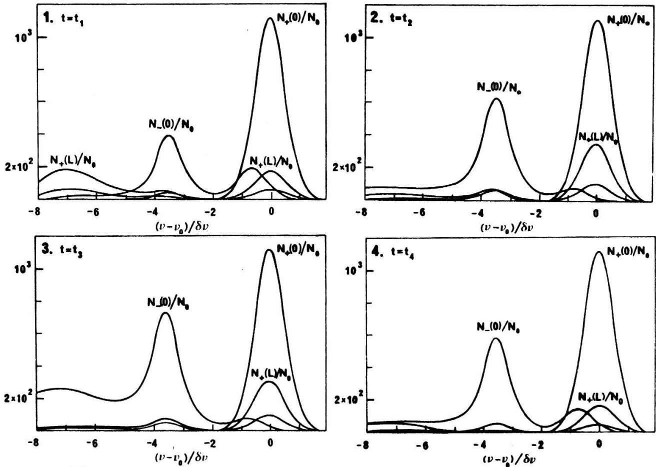
Fig. 3 Instantaneous radiation spectra N_{\pm}(\nu, x, t) for times shown in Fig.1
