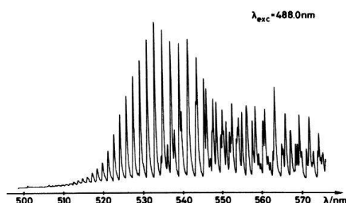
Fig. 1A : Fluorescence from free \text{I}_2 produced by the photodissociation of \text{I}_2\text{Xe} at 488 nm. P = 0,5 \text{ bar} , P(\text{I}_2) = 2 \text{ mbar} , T = 350 \text{ K} . The fluorescence observed is from v' = 20\text{--}46 to v'' = 0\text{--}3 .
