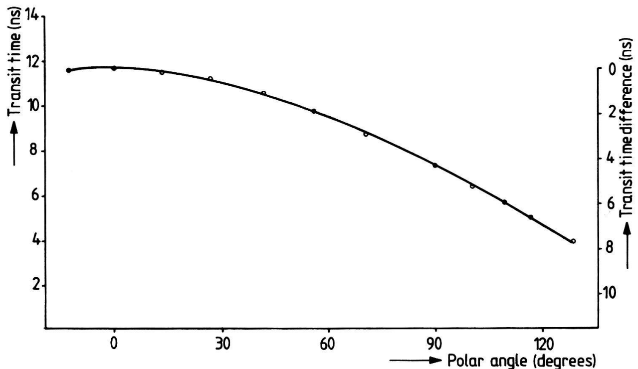
Figure 3. Transit time and transit time difference as a function of polar angle at 35 kV.
