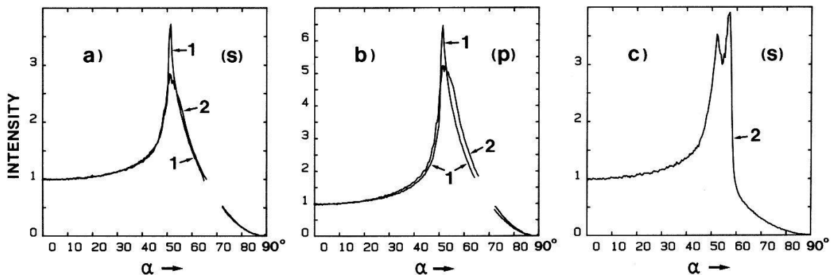
Fig. 4. (Normalized) angular distribution of evanescent-wave-induced luminescence I^{(s,p)}(\alpha) vs angle \alpha of liquid film (1), after solidification (2), for gap thickness a) and b) d_0 = 3.5 \mu\text{m} and c) d_0 = 1.2 \mu\text{m} . Normalization: I^{(s,p)}(\alpha=0) = 1 .
