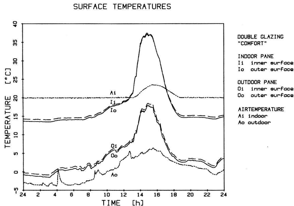
Fig. 3 In-situ measurements of indoor and outdoor air temperatures and surface temperatures of a double-glazed "Comfort" window measured thermoelements, recorded on March 11, 1986
