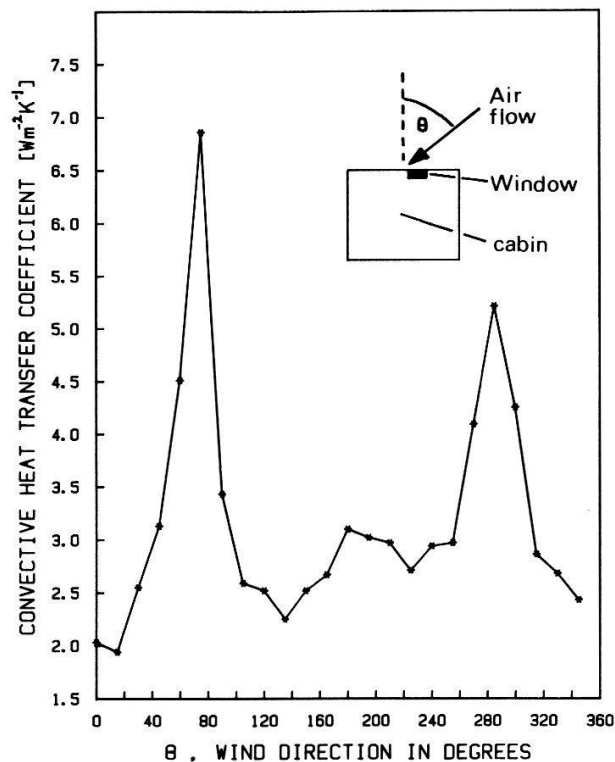
Fig. 3 Plot of convective heat transfer coefficient as a function of wind direction for real size cabin at 1 m/s
