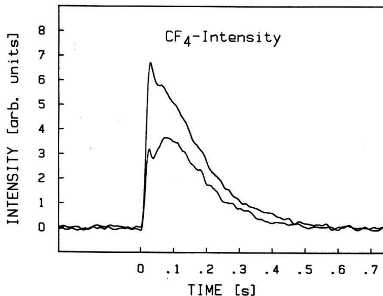
Fig. 3 Temporal evolution of the CF 4 concentration for two different geometrical arrangements of the PTFE nozzle.
