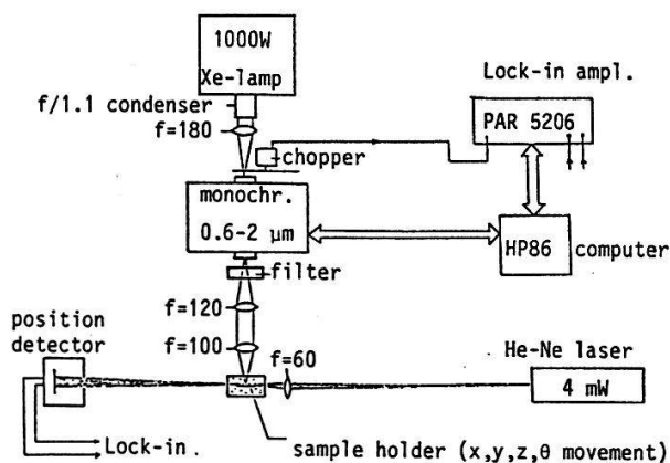
Fig.2 Setup for transversal PDS.
