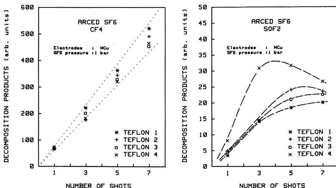
Fig. 1 Concentration of \text{CF}_4 and \text{SOF}_2 as a function of the cumulated arc energy which is proportional to the number of shots
