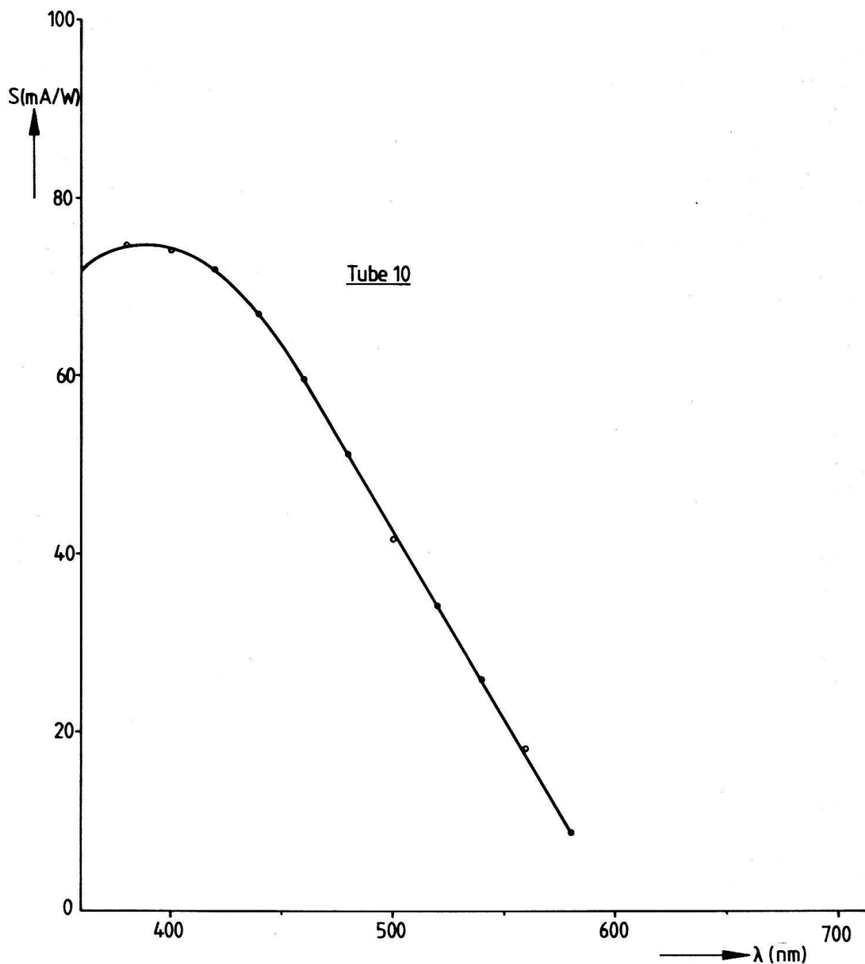
Figure 4. Spectral sensitivity characteristic of the preamplifier tube.
