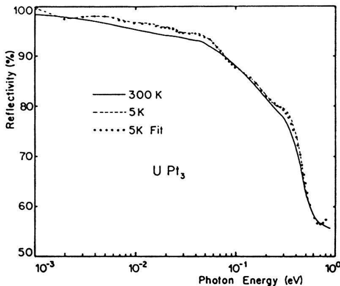
Fig. 1 : Near normal incidence reflectivity of \text{UPt}_3 at 5 K and at 300 K. Dots correspond to the fit with Lorentz oscillators.
