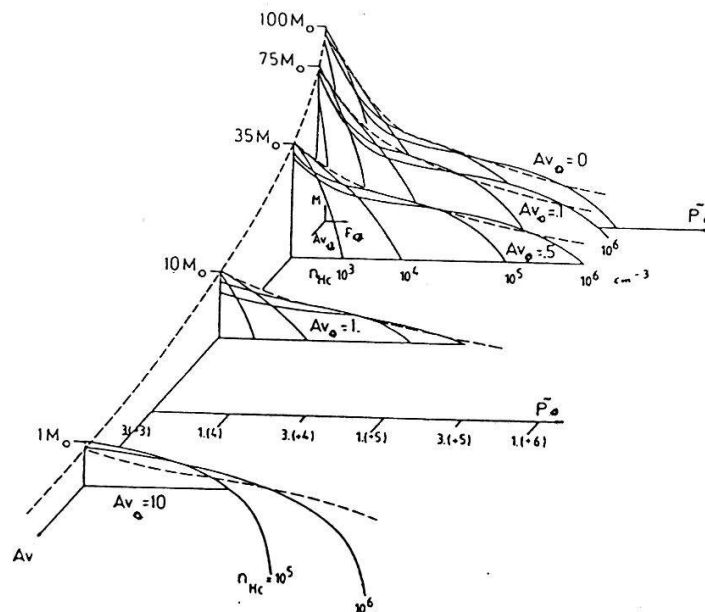
Figure 1. The stability domain of molecular cores in the (M, P_0, A_v) space.
