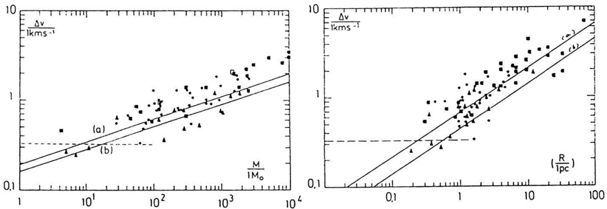
Fig.2: The internal velocity dispersion as a function of the mass and the radius of the clouds and their condensations.
