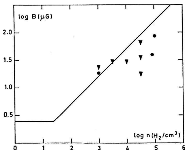
Fig. 1 The Nançay OH Zeeman results for the measured magnetic fields in molecular clouds plotted against the estimated gas densities of clouds. Filled circles correspond to detected fields and downward pointing triangles correspond to upper limits at the upper limit value. The line is a simplified version of the theoretical predictions (2).
