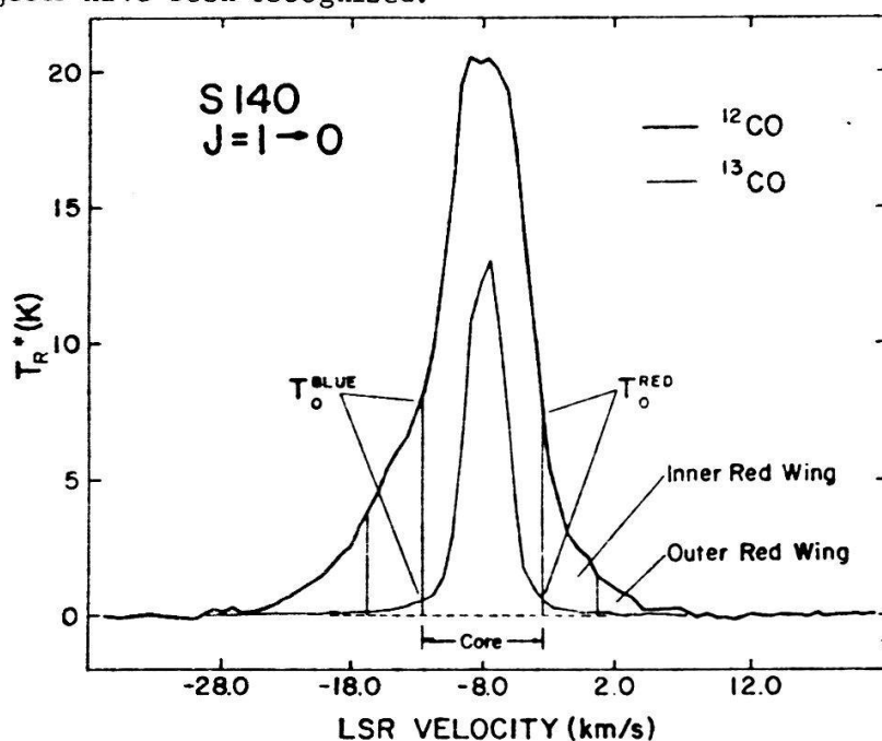
Figure 1 : example of a ^{12}\text{CO} spectrum with high-velocity wings (from (1))
