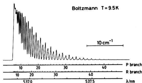
Fig. 3B : Computer simulation of 3A for \text{I}_2(\text{B}) rotational temperature of 9.5 K assuming Boltzmann distribution.
