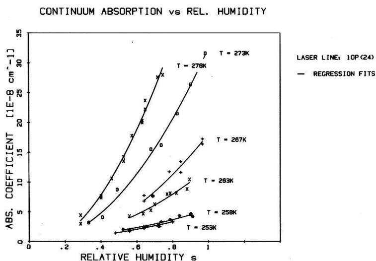
Fig. 1 Measured continuum absorption versus relative humidity at the 10P(24) \text{CO}_2 -laser transition.
