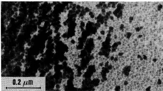
Fig. 4b: This TEM picture is an enlargement of a section at the fringe of Fig. 4a showing the microscopic structure of the deposited Ga. The particles are quite spherical, have a diameter between 10 and 20 nm and are amorphous.
