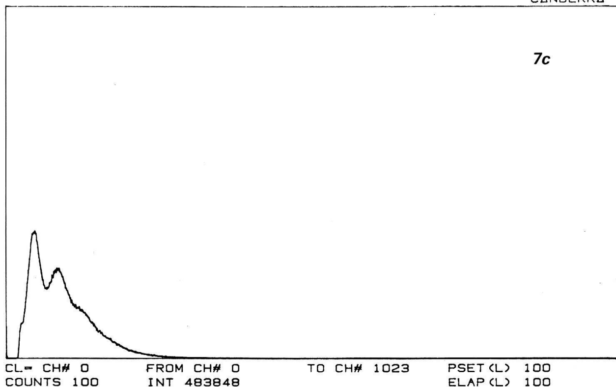
Figure 7. Pulse height distributions for 15 kV (a), 25 kV (b) and 30 kV (c) with low light pulse intensity.
