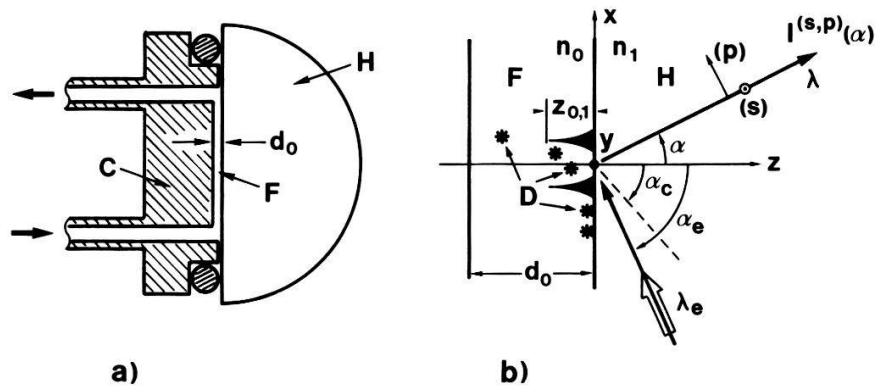
Fig. 1. a) Schematic of dye cell: H, hemicylindrical high index ( n_1=1.89 ) glass prism (LASF15); C, cell; thickness of liquid film F typically d_0 \approx 10 \mu\text{m} ; b) \alpha_e , angle of incidence of exciting laser beam of wavelength \lambda_e ; z_{0,1} , penetration depth of evanescent wave; n_0 , refractive index of dye solution; D, dye molecules; \alpha_c = \arcsin(n_0/n_1) ; \alpha , angle of emission of luminescent light of wavelength \lambda ; I^{(s,p)}(\alpha) , angular intensity distribution of luminescent light; (s), (p), polarizations.
