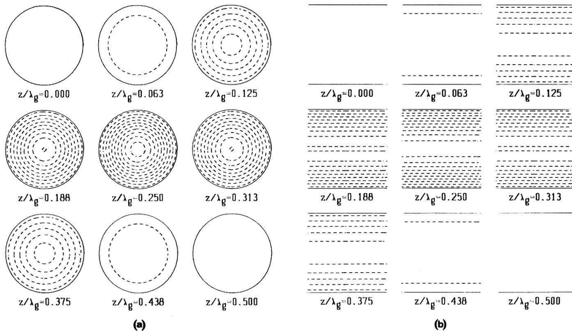
Fig. 3 Contours of the longitudinal electric field for an eigenmode of the TM_{01}/TM_{01} coupling at the lower stopband edge. For a particle with velocity equal to the phase velocity of the eigenmode.
