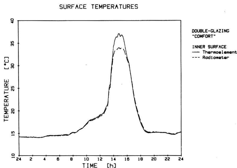
Fig. 2 Indoor surface temperature of a double-glazed "Comfort" window measured by a thermoelement and by a 8 to 14\ \mu\text{m} radiometer on March 11, 1986
