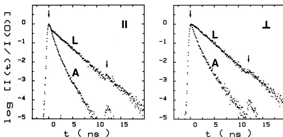
Fig. 6. Decay of luminescent intensity of sulforhodamine 101 versus time t (measured by time correlated single photon counting). Excitation \lambda_e = 565 nm, emission \lambda = 600 nm; polarizations in emission and excitation parallel (II), and orthogonal ( \perp ). Dye molecules in bulk solution (L), and adsorbed on glass surface (A). 1/e -decay-times: \tau_L'' = 3.7 ns, \tau_L^\perp = 4.9 ns, \tau_A'' = 1.3 ns, and \tau_A^\perp = 1.6 ns. Arrows indicate the positions of the main excitation pulse and of a weak second pulse.
