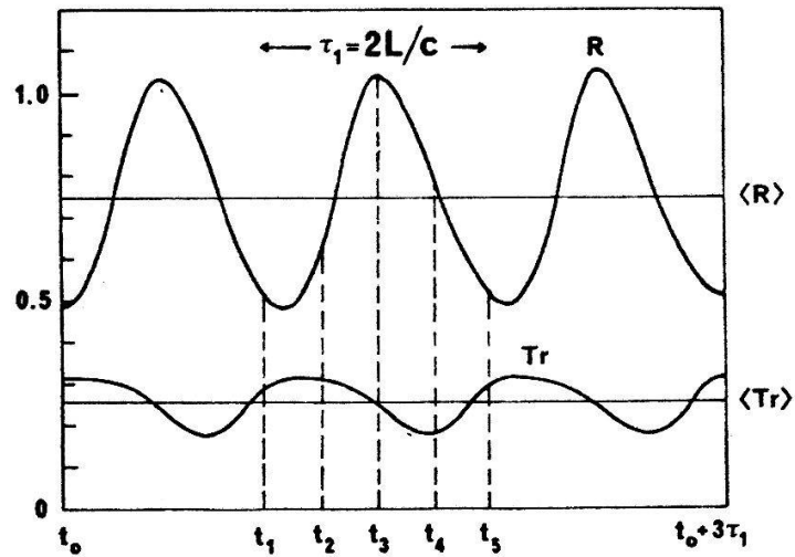
Fig. 1 Steady self-oscillations of the reflection R and transmission Tr coefficients obtained from Eqs. (2) and boundary conditions (12) for r_{in} = r_{out} = 0.2
