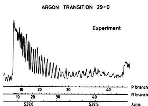
Fig. 3A : Rotationally resolved fluorescence spectrum following \text{I}_2\text{Ar} dissociation at 488 nm. Observation on the 29-0 vibrational transition.
