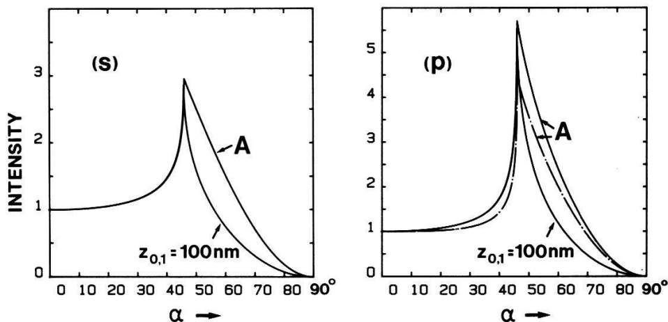
Fig. 4 a,b. Calculated radiation patterns I^{(s,p)}(\alpha) versus \alpha for ensemble of randomly oriented electric dipoles: (A) adsorbed on the interface 0/1; ( z_{0,1} ) located in the solution, excited with evanescent wave of penetration depth z_{0,1} = 100 nm. n_0 = 1.36 , n_1 = 1.89 . (— · — · —) radiation pattern as (A) for non-isotropic dipole orientation (see text).
