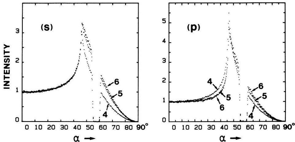
Fig. 3. Measured radiation patterns I^{(s,p)}(\alpha) of rhodamine 6G in ethanol ( n_0=1.36 ) at concentrations C = 5 \times 10^{-6} mole/liter (6), 5 \times 10^{-5} mole/liter (5) and 5 \times 10^{-4} (4), respectively. \alpha_e = 58^\circ ; penetration depth z_{0,1} = 100 nm; excitation: \text{Ar}^+ -laser \lambda_e = 514 nm; selected emission wavelength \lambda = 556 nm.
