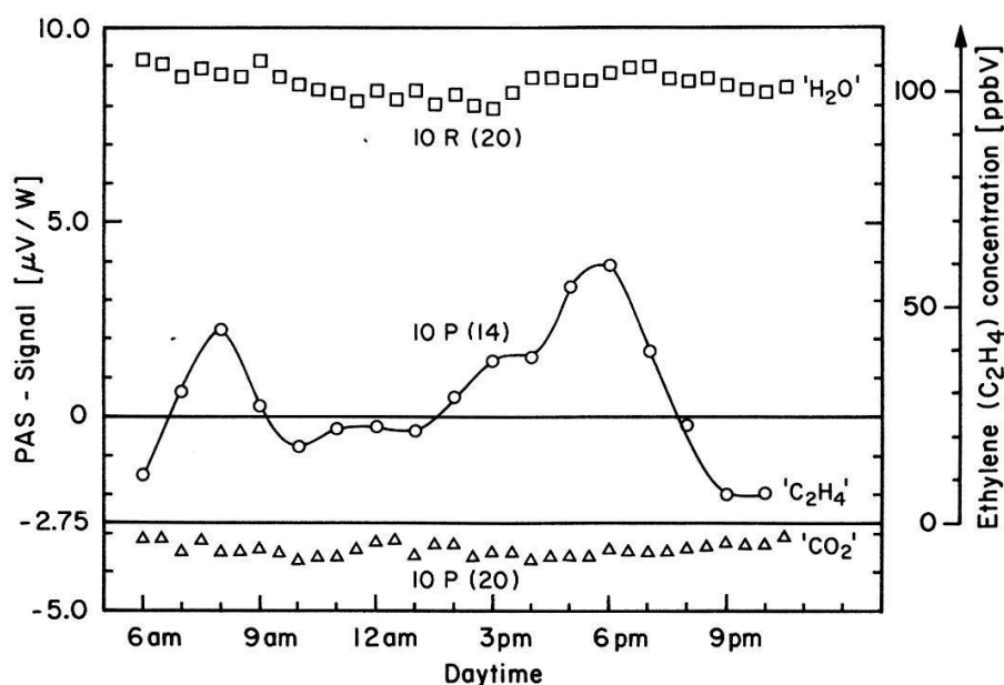
Fig. 2 PA signals for \text{H}_2\text{O} , \text{C}_2\text{H}_4 and \text{CO}_2 versus daytime. Date: Feb 4, 1986
