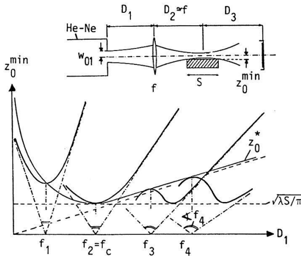
Fig.3 Minimum distance z_0^{\min} as function of focal length f , distance D_1 and laser beam parameters.
