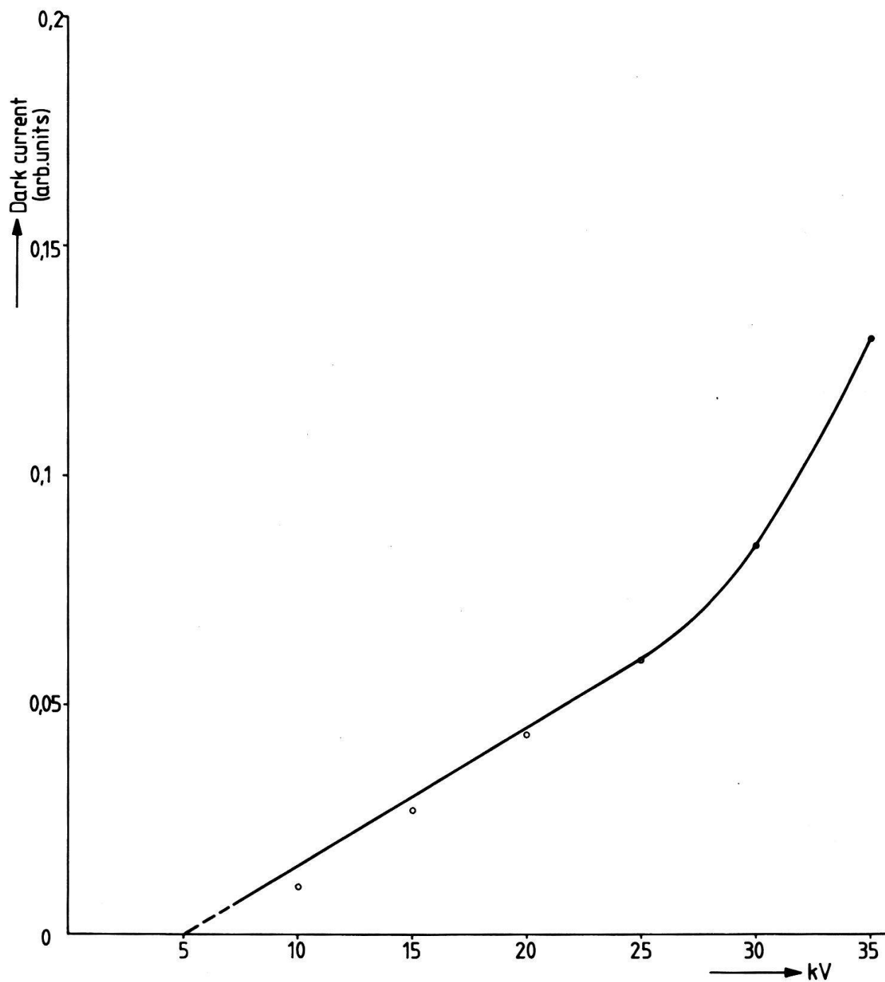
Figure 10. Dark current as a function of the accelerating voltage.
