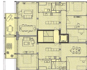
Grundriss Imphenia.
