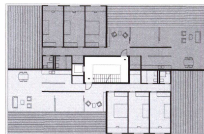
Attikageschoss
