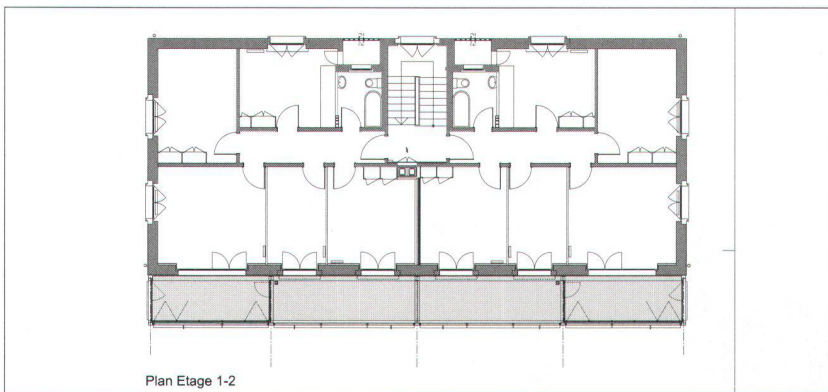
Plan Etage 1-2
