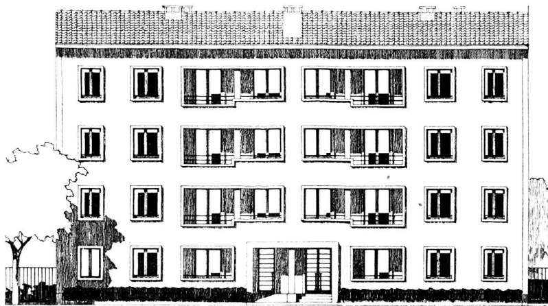
Façade principale. Molinié, Sarce, Cherenot, architectes.
