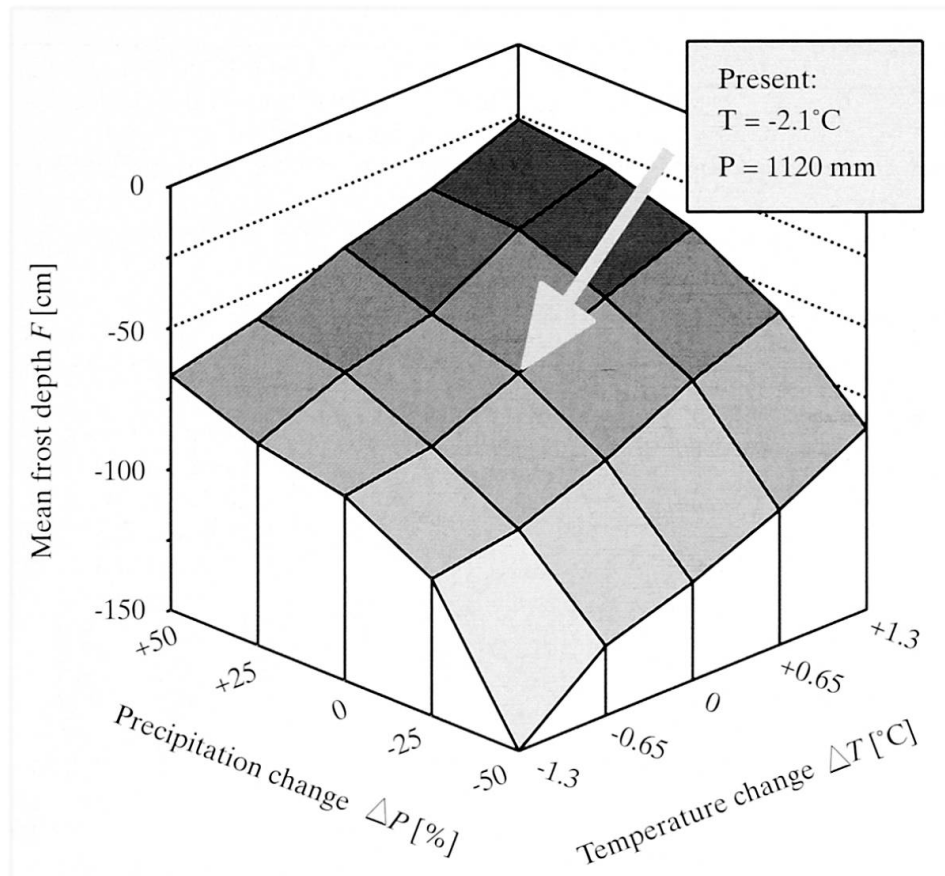
Fig. 8: Mean simulated frost depths occurring under systematically varied climatic conditions (see text)
