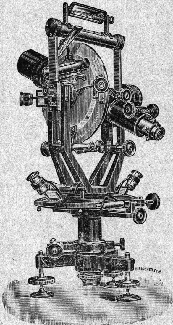
Repetitions-Theodolit 180/183
