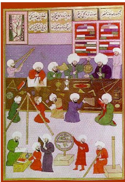
Astronomie in Istanbul 1577 Observatorium Taqī ad-Dīn
