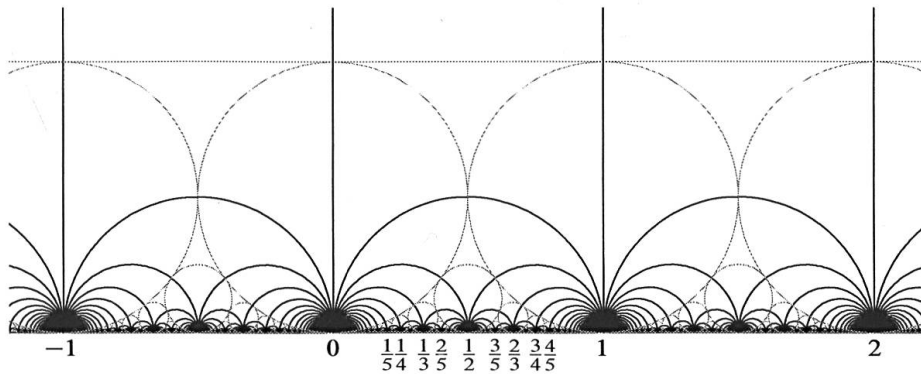
FIGURE 6 Ford circles and Farey tessellation
