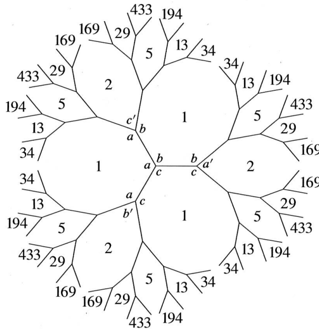
FIGURE 1 Markov tree
