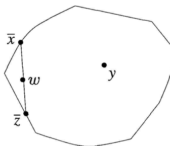
FIGURE 5 Partial hyperbolicity
