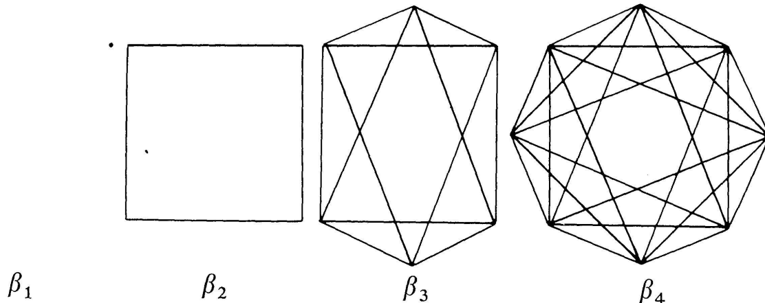
Cross Polytopes
