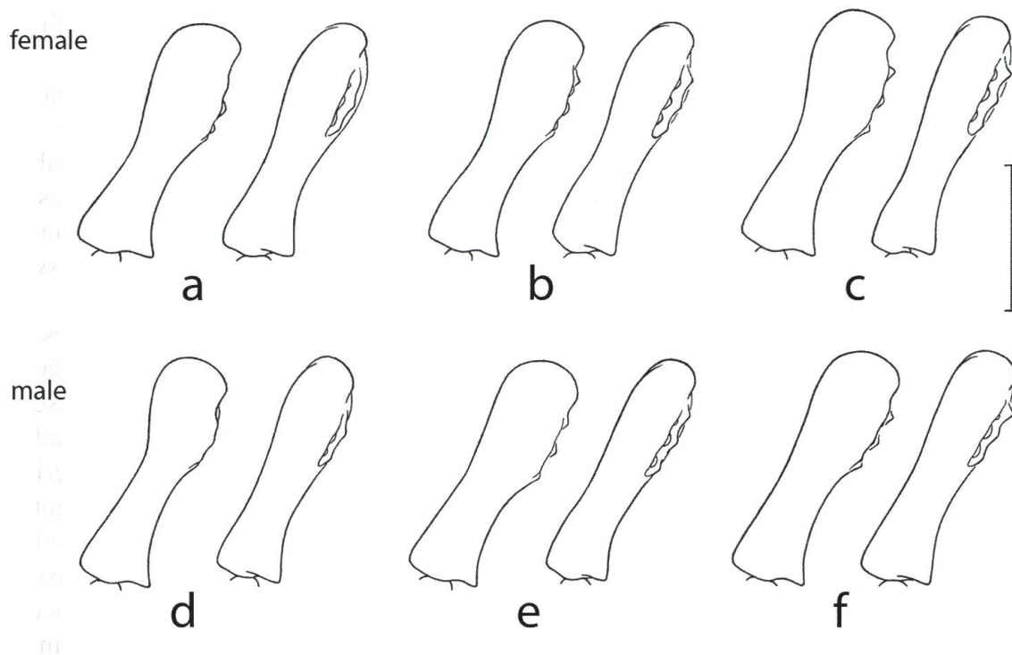
Fig. 6. Paussus brancuccii sp.nov., variation of antennal club, examples (cf. Fig. 5): dorsal view and view slightly rotated to the left through longitudinal axis; paratypes. Upper row, female specimens: a = Laos-NE, Houaphan prov., Phou Pane Mt., Ban Saleui env., 10.–22.V.2011 / 20°12'N 103°59'E, 1200–1600m, St. Jákl and Lao collectors leg.; b = Laos-NE, Houa Phan prov., 20°13'30"N 103°59'30"E, Ban Saleuy village env., 15–22.vi.2011, ~1350m, Vít. Kubáň & Lao coll. leg. / Secondary mountain forest, individual collecting, Laos 2011 Expedition, National Museum Prague, Czech Republic; c = Laos-NE, Houa Phan prov., 20°13'30"N 103°59'30"E, Ban Saleuy village env., 15–22.vi.2011, ~1350m, Vít. Kubáň & Lao coll. leg. / Secondary mountain forest, individual collecting, Laos 2011 Expedition, National Museum Prague, Czech Republic. Lower row, male specimens: d = Laos-NE, Houa Phan prov., 20°13'30"N 103°59'30"E, Ban Saleuy village env., 15–22.vi.2011, ~1350m, Vít. Kubáň & Lao coll. leg. / Secondary mountain forest, individual collecting, Laos 2011 Expedition, National Museum Prague, Czech Republic; e = Laos-NE, Houa Phan prov., 20°13'30"N 103°59'30"E, Ban Saleuy village env., 14–24.vi.2012, ~1350m, Vít. Kubáň & Lao coll. leg. / Secondary mountain forest, individual collecting, Laos 2012 Expedition, National Museum Prague, Czech Republic; f = Laos-NE, Houaphan prov., Phou Pane Mt., Ban Saleui env., 10.–22.V.2011 / 20°12'N 103°59'E, 1200–1600m, St. Jákl and Lao collectors leg. Scale = 1 mm (illustration E. Weber).
