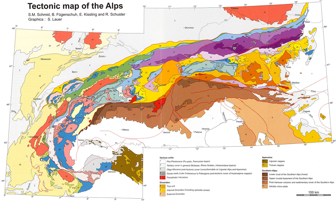
Plate 1 Tectonic map of the Alps S.M. Schmid et al.
