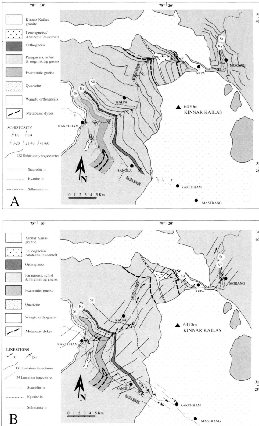
Fig. 6. Geological map of the area of study (geology and metamorphic isogrades based on Vannay & Grasemann (1998) and our own observations). A: D2 schistosity trajectories map. B: D2 stretching lineation trajectories.
