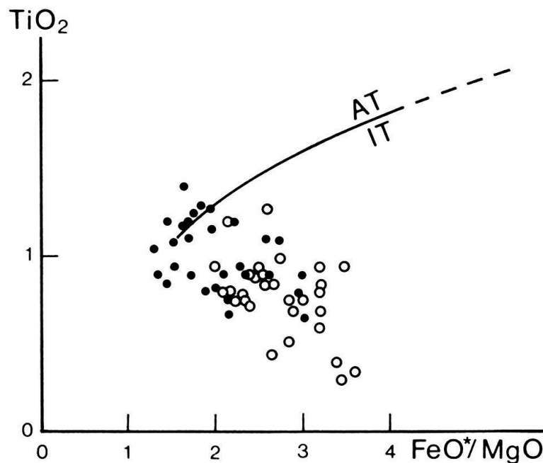
Fig. 1. TiO 2 -content versus FeO*/MgO ratio in Middle Triassic volcanic (full circles) and basic intrusive rocks (open circles) of the Dolomites, Southern Alps. IT = isotitaniferous "orogenic"; AT = anisotitaniferous "anorogenic" association fields (BÉBIEN 1980). Note the negative correlation mainly in the intrusive sample distribution: i.e. a trend typical for the calc-alkaline series.
