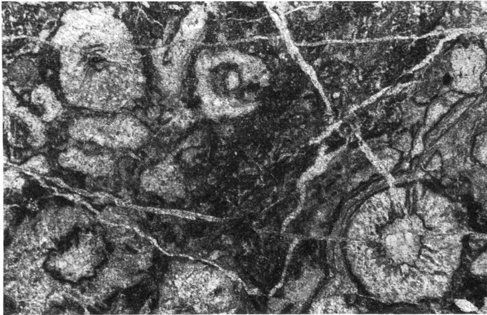
Fig. 10. Strongly "recrystallized" skeletal limestone with large dasyclad algae, Thaumatoporella . Gereme Limestone, Lower Jurassic, Unia Nisia, DB 1612. Thin-section. \times 4.5 .
