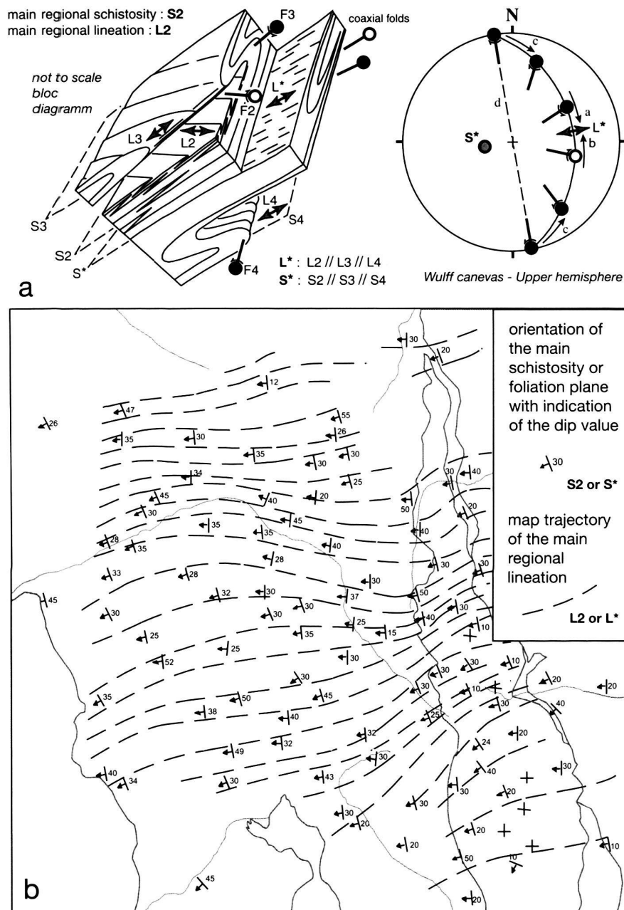
Fig. 4. The isoclinal structure of the Queyras Schistes lustrés. a: synthetic block diagram and stereonet showing the geometrical relationships between the folds (F), schistosity (S) and lineations (L) associated with the successive D2, D3 and D4 deformation phases. For clarity, the original flat-lying S1 foliation and the associated F1 isoclinal folds have been omitted (see "sandwiched marbles" in section YY', Plate 1). As proposed by Hansen (1971), arrows turning around the fold axis symbols indicate the asymmetry patterns of folds in terms of rotation of short limbs relative to long limbs about their hinge lines, the folds being observed down-plunge of the hinge line. The double grey arrows recall the importance of stretching along the successive generations of lineations. The L2 lineation is deformed around the hinge of a F3 fold. Just below, in a zone of accentuated D4 deformation, the earlier formed schistosity become parallel to S4, resulting in a single planar structure S*. The earlier formed stretching L2 and L3 lineations rotate within this plane S* and become parallel to the L4 stretching lineation, resulting in a single very strong stretching lineation L* of composite origin. After a comparable rotation (arrows a and b in the stereonet), the axes of the F2 and F3 folds also become parallel to L* (coaxial folds). Another consequence (not represented in the block diagram) is that the axes of the F4 folds, dominantly small-scale folds, leave their initial N-S horizontal orientation and start rotating (arrows c in the stereonet) within S4 toward the L4 direction of stretching, resulting in axes with a planar dispersion and hinges with a non-cylindrical geometry. In the stereonet, the dashed line (d) represents the projection of the plane of the section YY' (Plate 1). b: regional orientation of the dominant schistosity and lineation (same structural sketch map as in Fig. 2).
