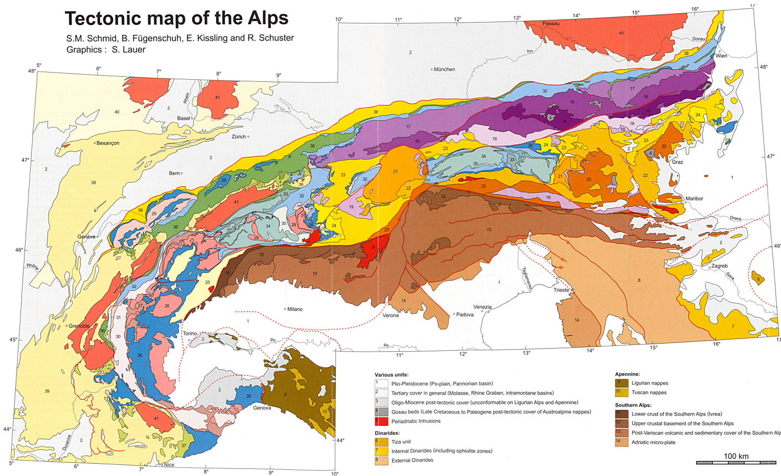
Plate 1 Tectonic map of the Alps
