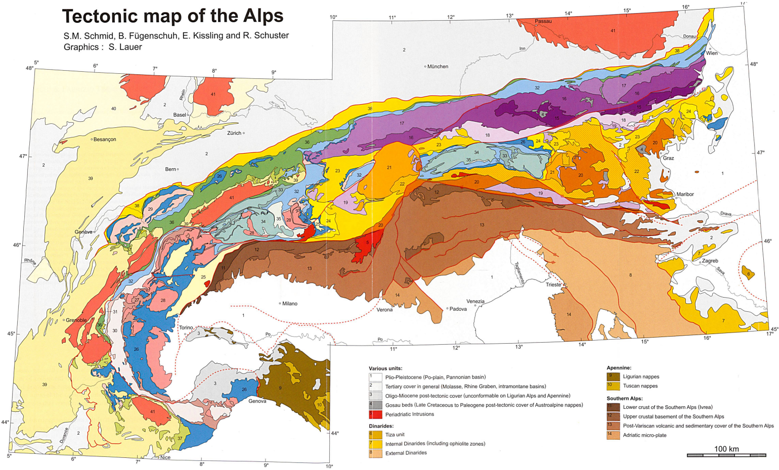
Plate 1 Tectonic map of the Alps
