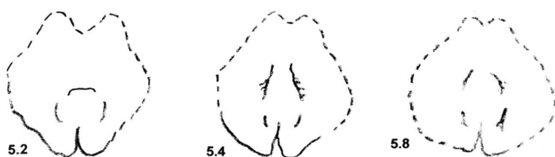
Fig. 12. Gemmarcula? plattenwaldensis sp. nov. Transverse serial sections of a specimen (length = 10.5 mm, width = 10.1 mm, thickness = 9.0 mm) from Plattenwald. Numbers give distance in mm from the posterior end. 3 \times nat. size.
