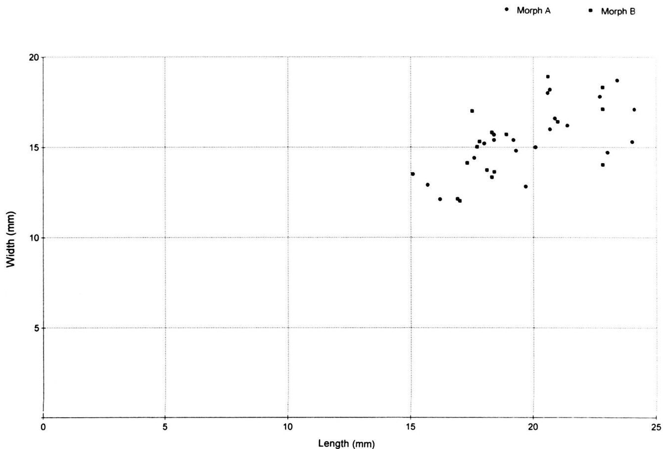
Fig. 10. Same population of Moutonithyrus dutempleana (d'Orbigny) as in fig. 9. Shell length and width of 21 specimens of morph A (width:length ratio = 0.64–0.89) and 16 specimens of morph B (width:length ratio = 0.69–0.97).
