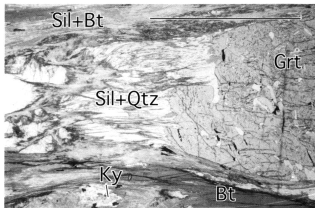
Fig. 13. Section parallel to D3 stretching lineation and fold axis. Synkinematic Qtz-Sil-aggregates indicate deformation in the sillimanite field. Phengite is almost completely decomposed to biotite in this sample (upper Val Grono). Width of scalebar is 5 mm.
