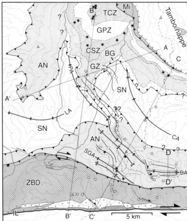
Fig. 4. Structural maps of the study area. The data are compiled from Hänni (1972), Weber (1966), Codoni (1981), Knoblauch et al. (1927), Bruggmann (1965), Kündig (1926), Bellin (1929), Jeker (2000), Niederberger (2000), Frischbutter (2000), Damo (2000) and this investigation. Legend is the same as for Fig. 3.
