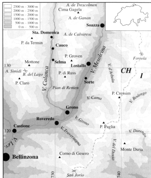
Fig. 2. Topographic reference map of the study area with all localities mentioned in the text. CH: Switzerland; I: Italy; circles: towns/villages; triangles: peaks; Coordinates are from the Swiss national topographic map grid.
