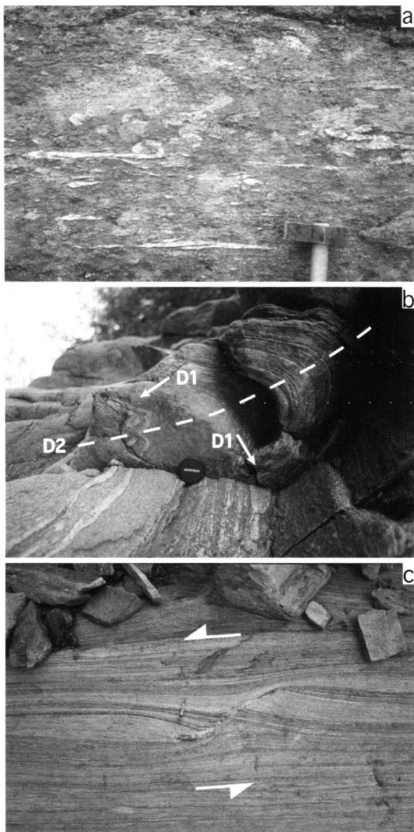
Fig. 6. Photographs illustrating D1 structures: (a) Isoclinal dismembered D1 folds in metapelites (Alp Calvares/ Calanca), refolding a pre-D1 foliation. (b) Isoclinal D1 folds, refolded by a tight D2 fold. Lower Auriglia-gorge (Selma, Calanca). (c) Shear band and associated oblique boudinage in Kfs-gneisses indicating a sinistral shear sense (= top N; Pass de Ganan, Calanca).
