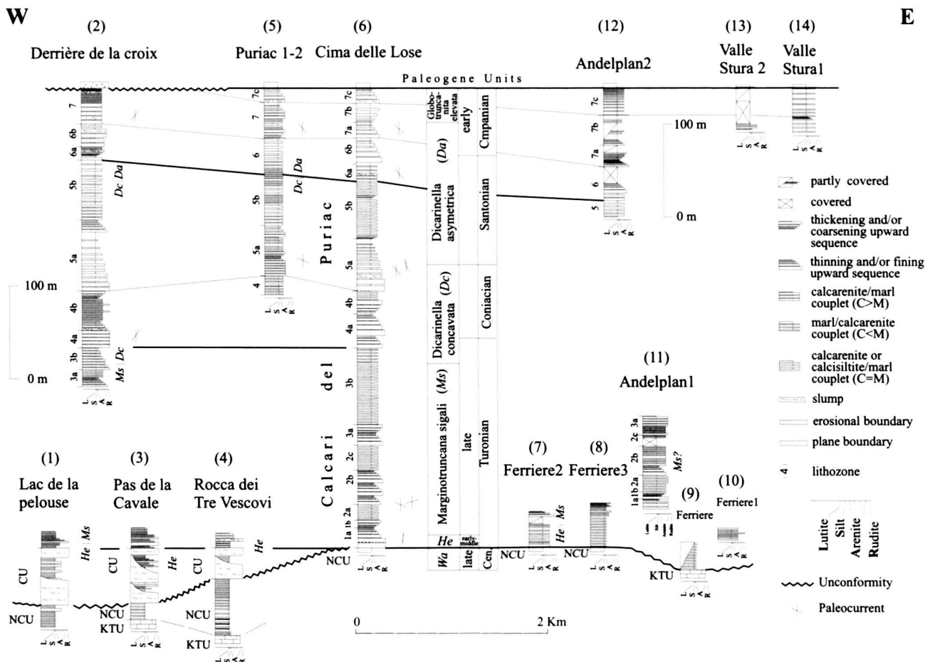
Fig. 3. Stratigraphy of the Helvetic Cretaceous succession in the upper Stura - Haute Ubaye area. Location of sections is reported in Fig. 2. Wa: Whiteinella archaeocretacea Zone; He: Helvetoglobotruncana helvetica Zone.
