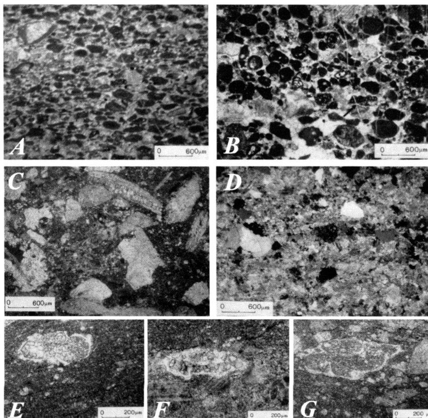
Fig. 6. Some microfacies of the Calcare del Puriac . (A) Ooidal – bioblastic grainstone with peloids and coated grains (Section Ferriere 2, lithozone 1b, facies gC); (B) grainstone/packstone with crinoids, echinoids, benthonic foraminifers (arrow indicates an orbitolinid) and ooids (Section Andelpan 1, lithozone 3a, facies C); (C) Skeletal packstone with rudist fragments and echinoderms (Section Derrière de la Croix, lithozone 4a, facies glCM); (D) calcarenite with mono- and polycrystalline quartz, lithics (chert, micritic limestones) bioclasts (echinoderms) and micritic intraclasts (Section Andelpan 2, lithozone 6, facies glCM). (E) Wackestone with D. algeriana , lithozone 1. (F) Wackestone with M. sigali , lithozone 3. (G) Wackestone with D. concavata , lithozone 5.
