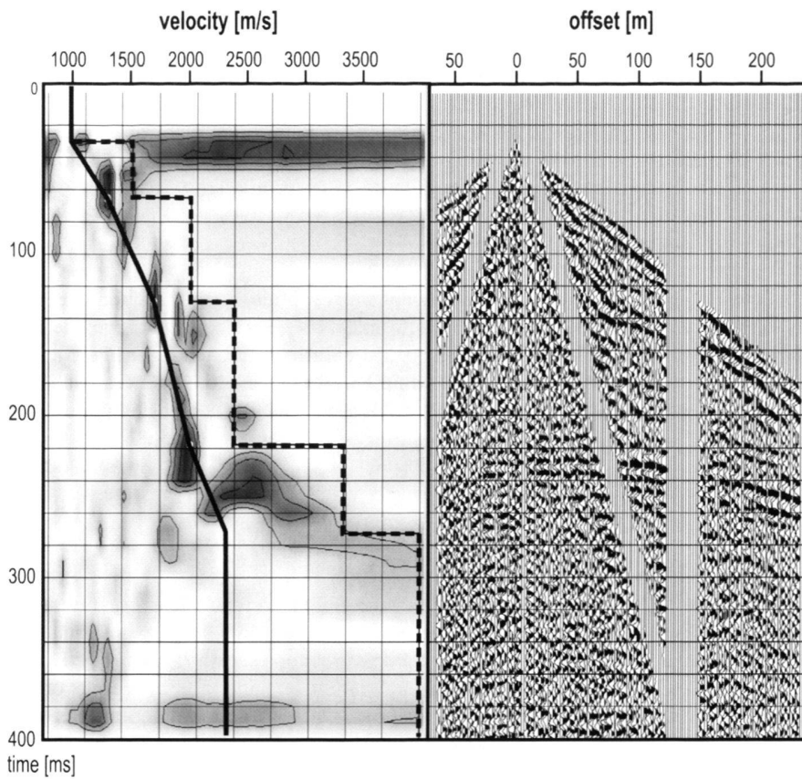
Fig. 5. Velocity panel of CMP 200 from Profile 1. Left side shows the semblance analysis with velocity picks and model. Right side shows the associated CMP supergather, a combination of three adjacent CMP's. Velocity picks were chosen based on a combination of maximum semblance, fitting of reflections on the CMP gather and optimum stacking results. Solid black line is the picked stacking velocity curve. Dashed line represents the resulting interval velocity.
