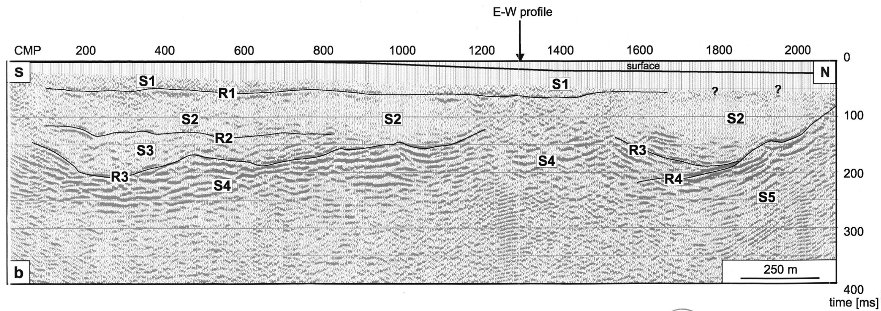
Fig. 6. (a) stacked section of Profile 1 (north-south profile). Note changes in amplitude character with increasing two-way traveltime. (b) Migrated section of (a) with interpreted units and main reflectors. Arrow on top marks the intersection with Profile 2 (E-W profile). For identification of units see text and Fig. 8.
