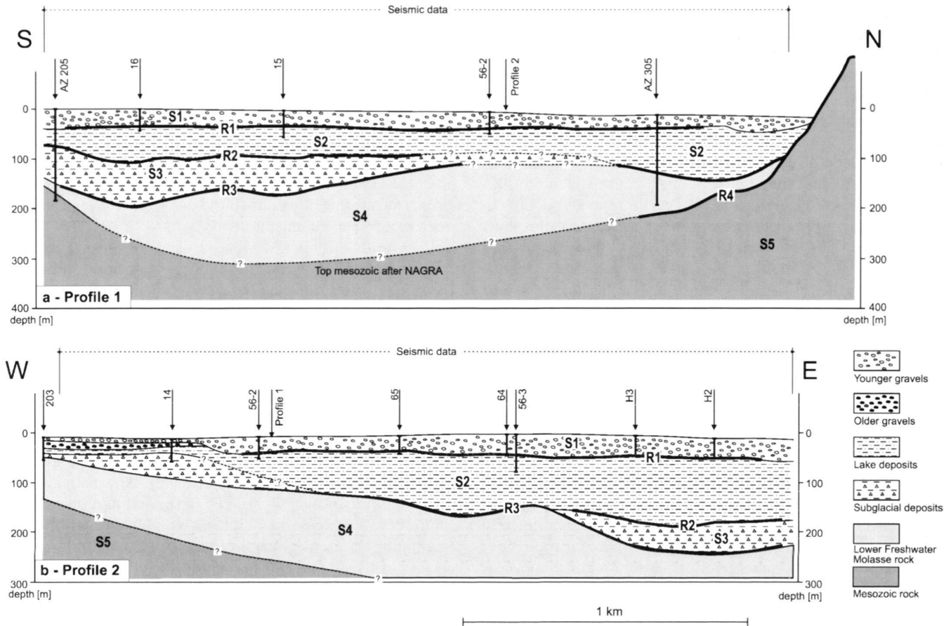
Fig. 8. Sketch of depositional model based on the interpretation of profiles 1 and 2 (Figs. 6 and 7) and borehole records. Information on Molasse-Mesozoic boundary is from the NAGRA profiles (Sprecher & Müller 1986) and borehole AZ-205. Note that several boreholes are projected from some distance to the profiles (Fig. 3). Thick black lines show the location of seismic reflections R1-R4 identified in the time sections of Figs. 6 and 7. S1-S5 represent the seismic units as described in Figs. 6 and 7 and in Table 3.
