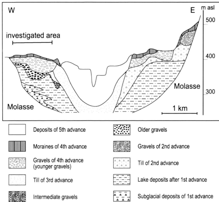
Fig. 2. Sketch demonstrating the schematic arrangement of infilling sediments in the Birrfeld area deposited by five different glaciations or glacial advances (after Graf, in press). It represents relative position and succession of erosional events based on outcrop and borehole information. The detailed shape and timing is not known.
