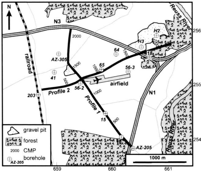
Fig. 3. Site map with detailed location of seismic profiles and boreholes. Highways and railroad tracks that encircle the study area are major sources of seismic background noise (borehole information by courtesy Matousek, Baumann & Niggli AG, Baden).
