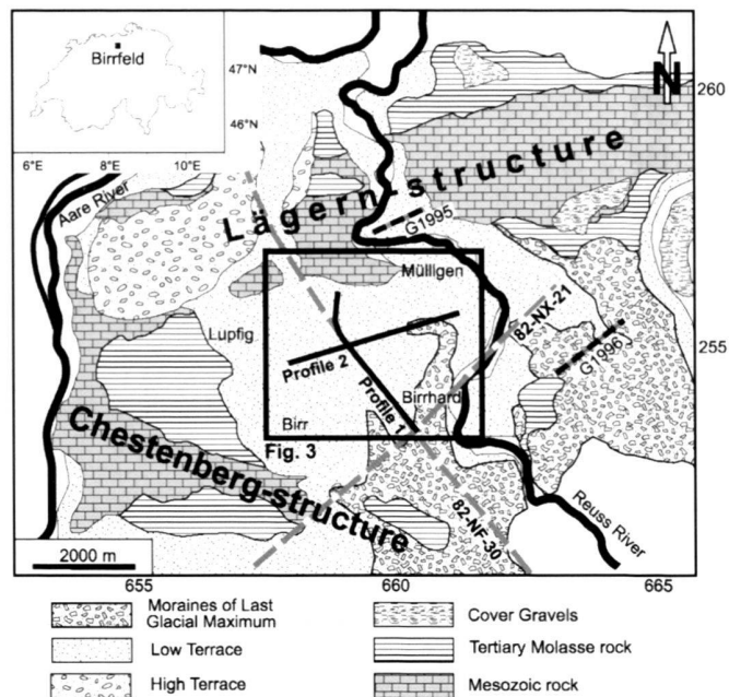
Fig. 1. Location and geological overview of the investigated area and surroundings. The Birrfeld area, enclosed by the rectangle, is enlarged in Figure 3. Location of earlier NAGRA seismic profiles (82-NF-30, 82-NX-21) is shown by gray dashed lines and location of GeoExpert lines (G1995, G1996) is shown by black dashed lines. Two continuous black lines indicate the position of the seismic reflection lines of this study. The Chestenberg- and Lägern-structures are anticline folds of the eastern part of the Jura mountain range. Coordinates around the main map refer to the Swiss reference system.
