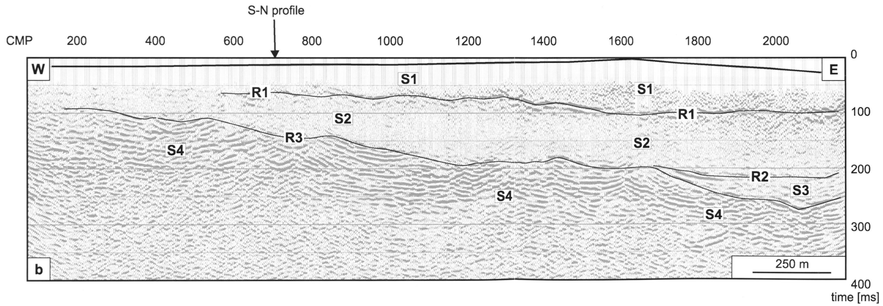
Fig. 7. (a) stacked section of Profile 2 (east-west profile). Note changes in amplitude character with two-way traveltime as in fig. 6a. (b) Migrated section of (a) with interpreted units and main reflectors. Arrow on top marks the intersection with Profile 1 (S-N profile). For identification of units see text and Fig. 8.
