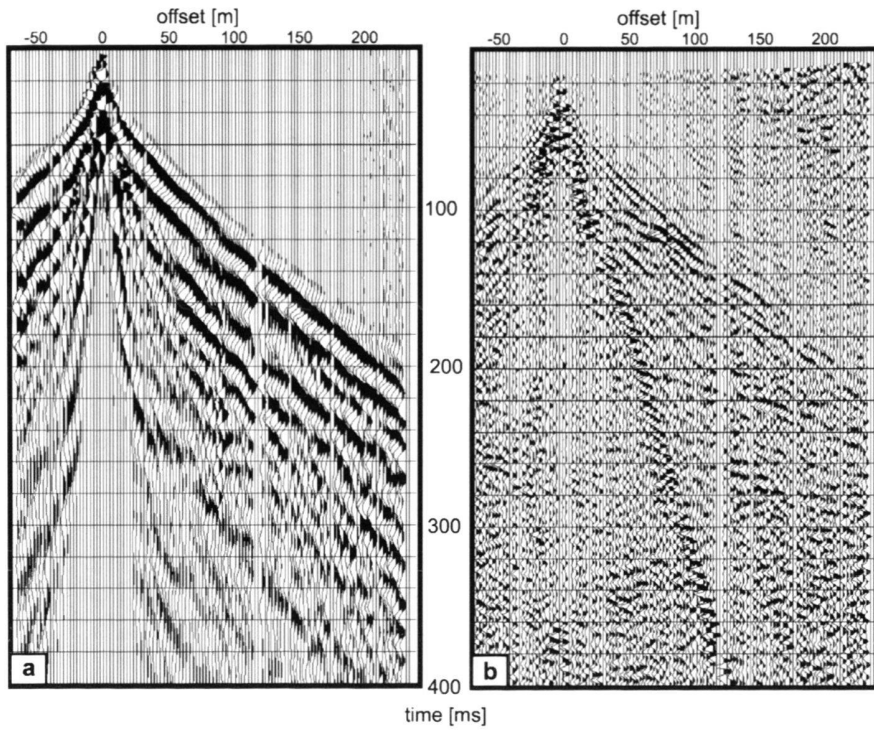
Fig. 4. Example of a shot gather of (a) raw data with only trace equalisation applied, and (b) the same data after applying initial processing including amplitude scaling, refraction static correction, spectral whitening, and frequency filtering.
