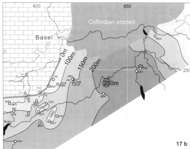
Fig. 17. Palinspastic reconstruction of both the Bärtschwil Fm. (Fig. left) and Effingen Member (Fig. right). Note that the basin depocenters shift from the north (Bärtschwil Formation) to the south (Effingen Member) over time and the coeval shallower environments also follow this relief inversion.
