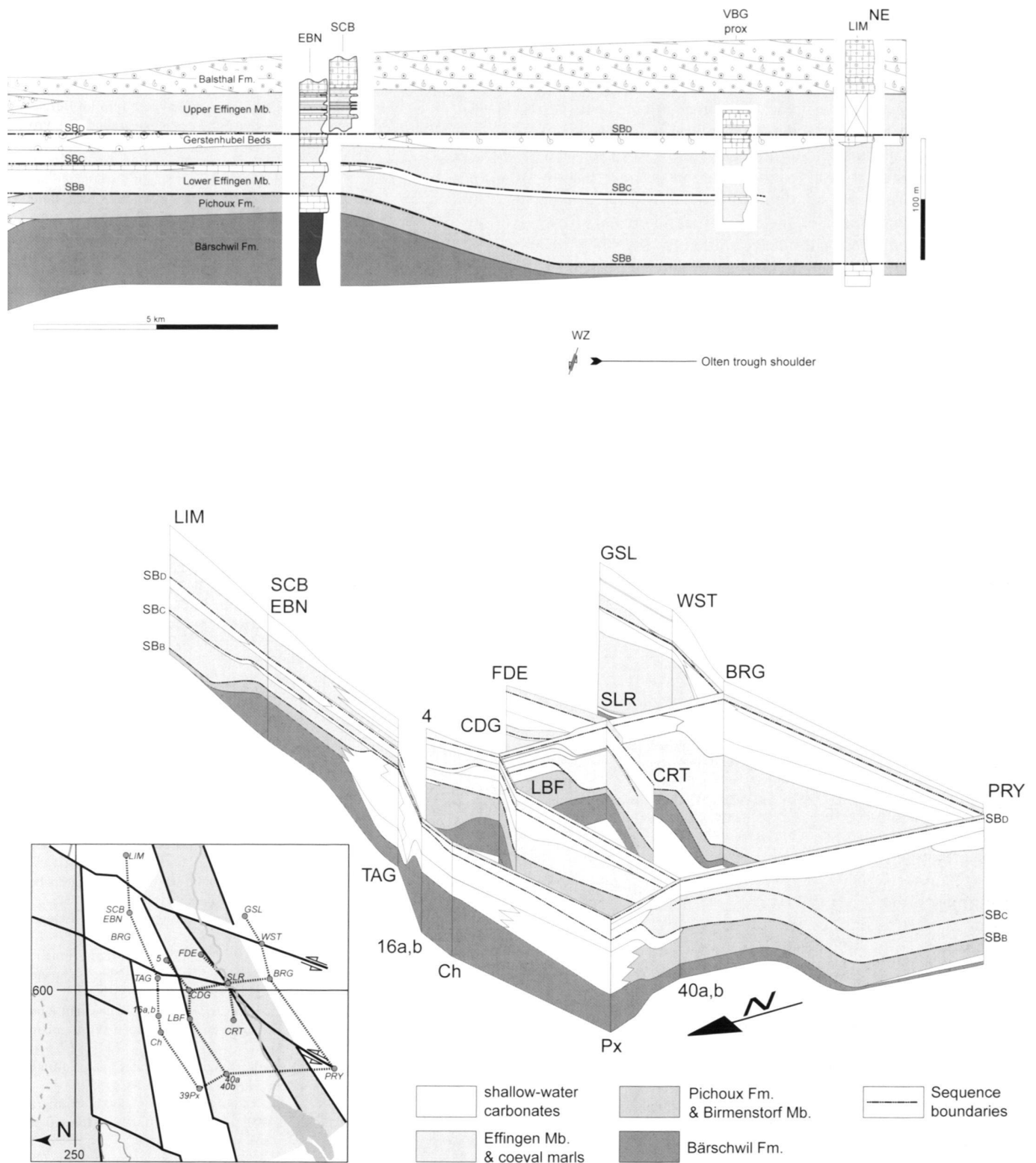
Fig. 22. This three-dimensional fence diagram shows the influence of Paleozoic faults (inset and Fig. 5) on the Mid Oxfordian environment. The profiles correspond to Figures 19–21 and Plate 1 and their positions are shown in the inset. Accommodation space is provided by differential subsidence along trough master-faults, while the Rhenisch lineament and northern Hermrigen trough masterfault also act as major facies-defining structures.
