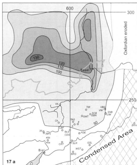
Fig. 17. Palinspastic reconstruction of both the Bärtschwil Fm. (Fig. left) and Effingen Member (Fig. right). Note that the basin depocenters shift from the north (Bärtschwil Formation) to the south (Effingen Member) over time and the coeval shallower environments also follow this relief inversion.
