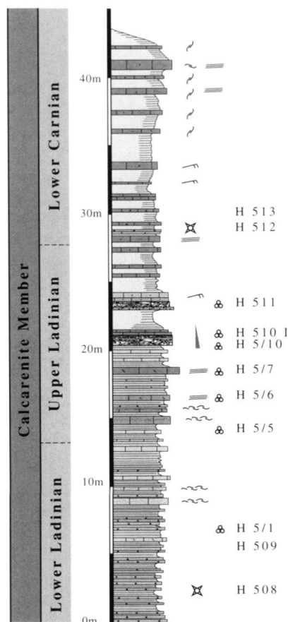
Fig. 6 A. Lithostratigraphy of a part of the calcarenite Member of the Sal Formation dominated by the characteristic filamentous limestones and Early Carnian radiolarian cherts.
