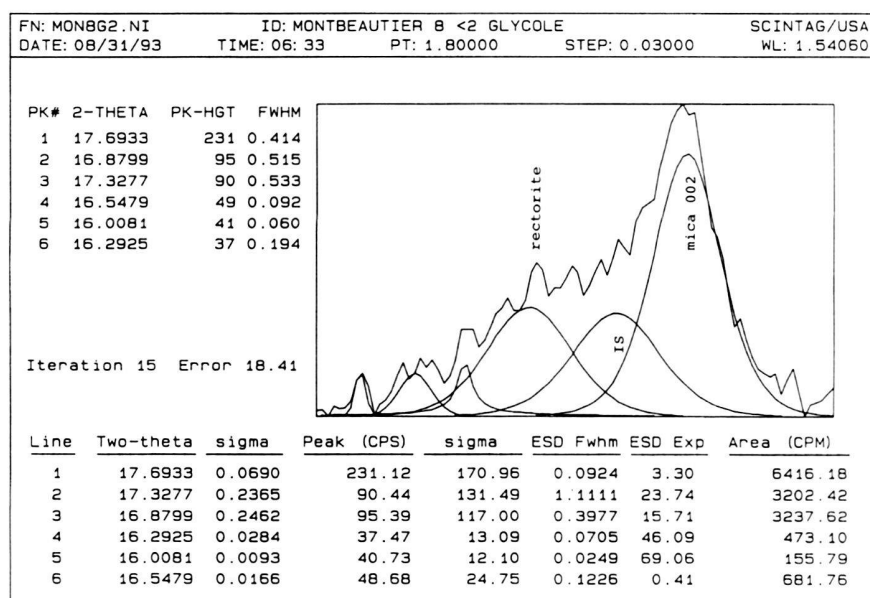
Fig. 13. X-ray diffraction pattern presenting reflections of mica 002, mixed-layers (IS) and rectorite between 16-17.7^{\circ}2\theta \text{CuK}\alpha_1 .
