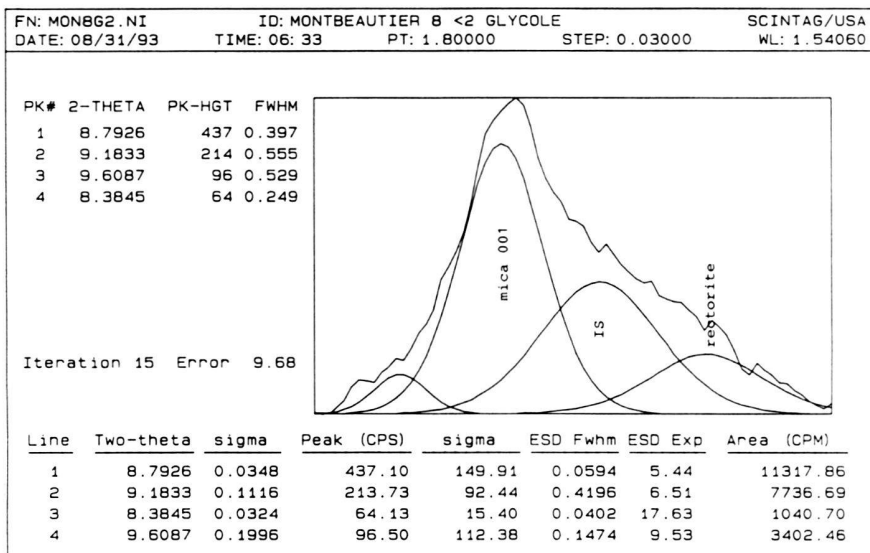
Fig. 12. X-ray diffraction pattern presenting reflections of mica 001, mixed-layers (IS) and rectorite near 10^{\circ}2\theta \text{CuK}\alpha_1 .
