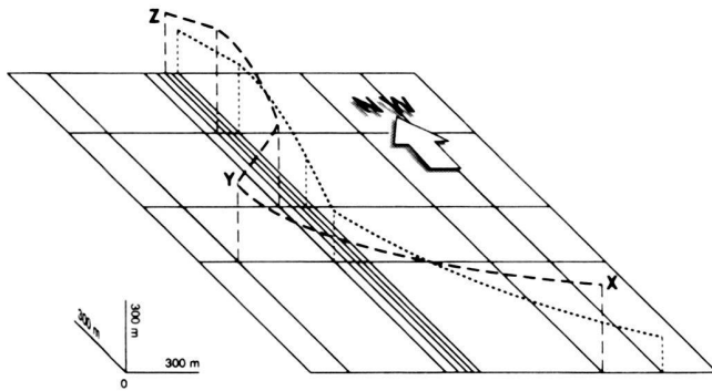
Fig. 2. Three-dimensional development of the hinge lines of the two D1 kilometre-scale folds (dashes: anticline; dots: syncline) that crop out on the south-western side of M. Camulera. See cross-sections 1, 2, 3 in Plate 1 for location of points X, Y and Z on the anticline hinge. The sheath-like geometry (more pronounced in the overlying anticline) is apparent. Also note that both lines are affected by vertical variations, which are connected with the D3 deformational event.
