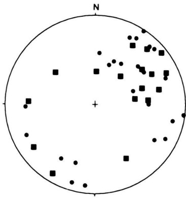
Fig. 3. Poles to 41 minor fault planes measured in some outcrops of the Mallore unit ( Ma1 and Ma3 formations). Dots and squares distinguish planes on which the pitch of striations is respectively high and low.
