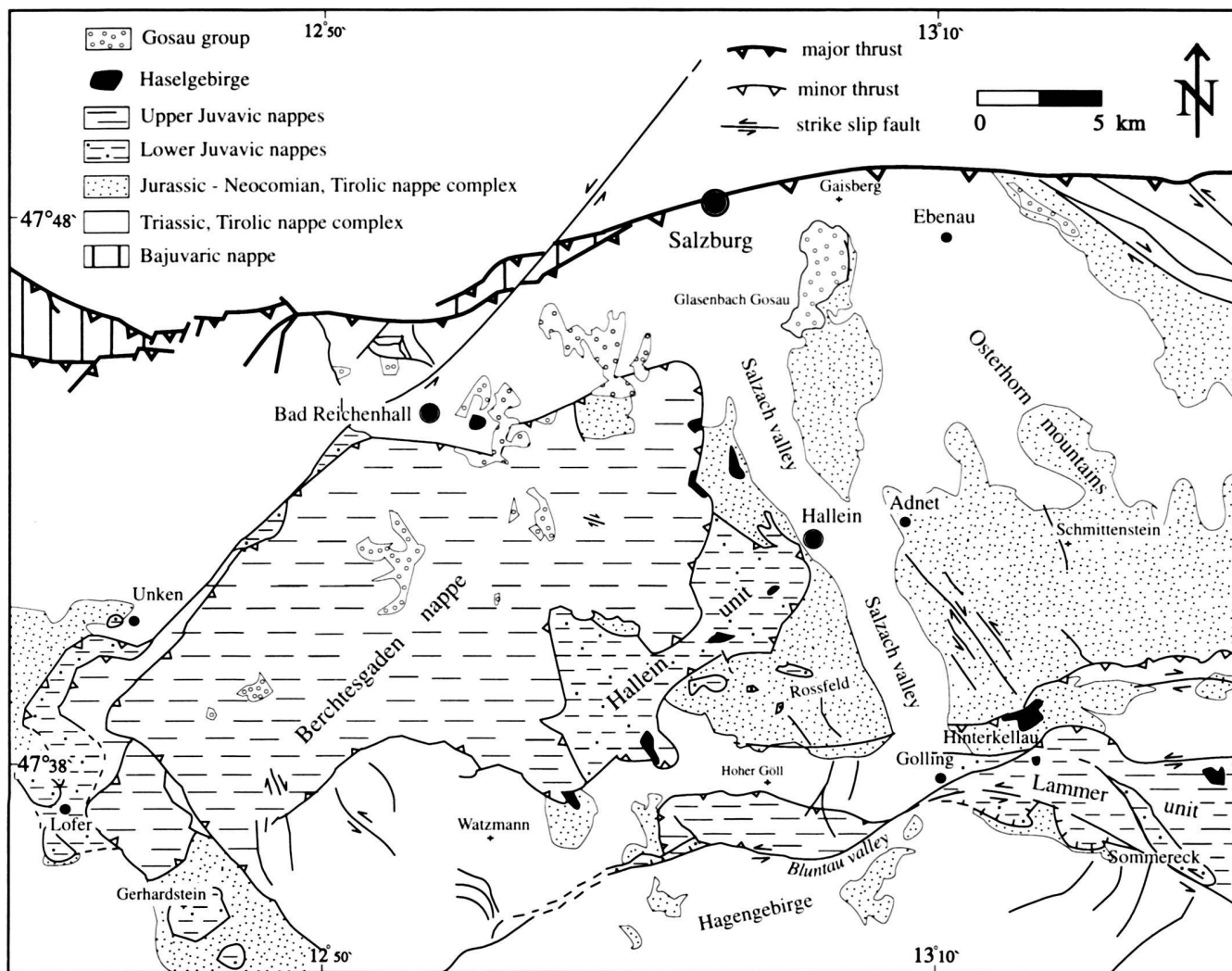
Fig. 2. Simplified geological map of the central NCA based on Ampferer (1927), Plöschinger (1982, 1987) and Prey (1969).
