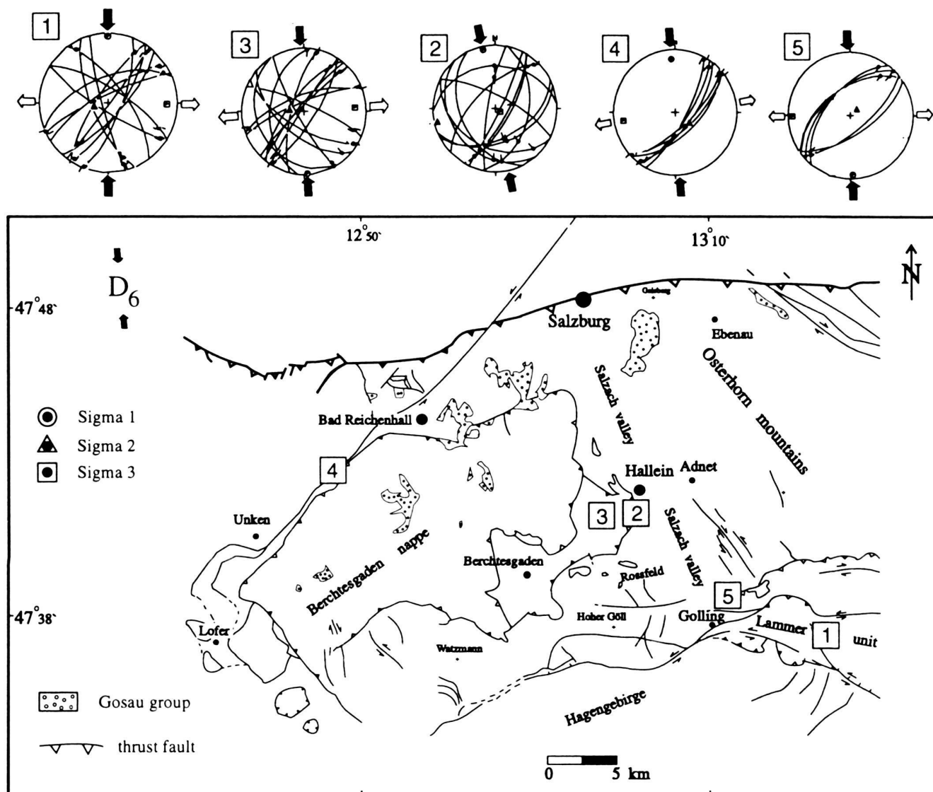
Fig. 15. Schmidt plots with faults and orientation of principal stress axes calculated by the right-dihedra method: a) Strike-slip, thrust and dip-slip faults dominate D_6 deformation, while b) D_7 is characterized by strike-slip and thrust-faults.
