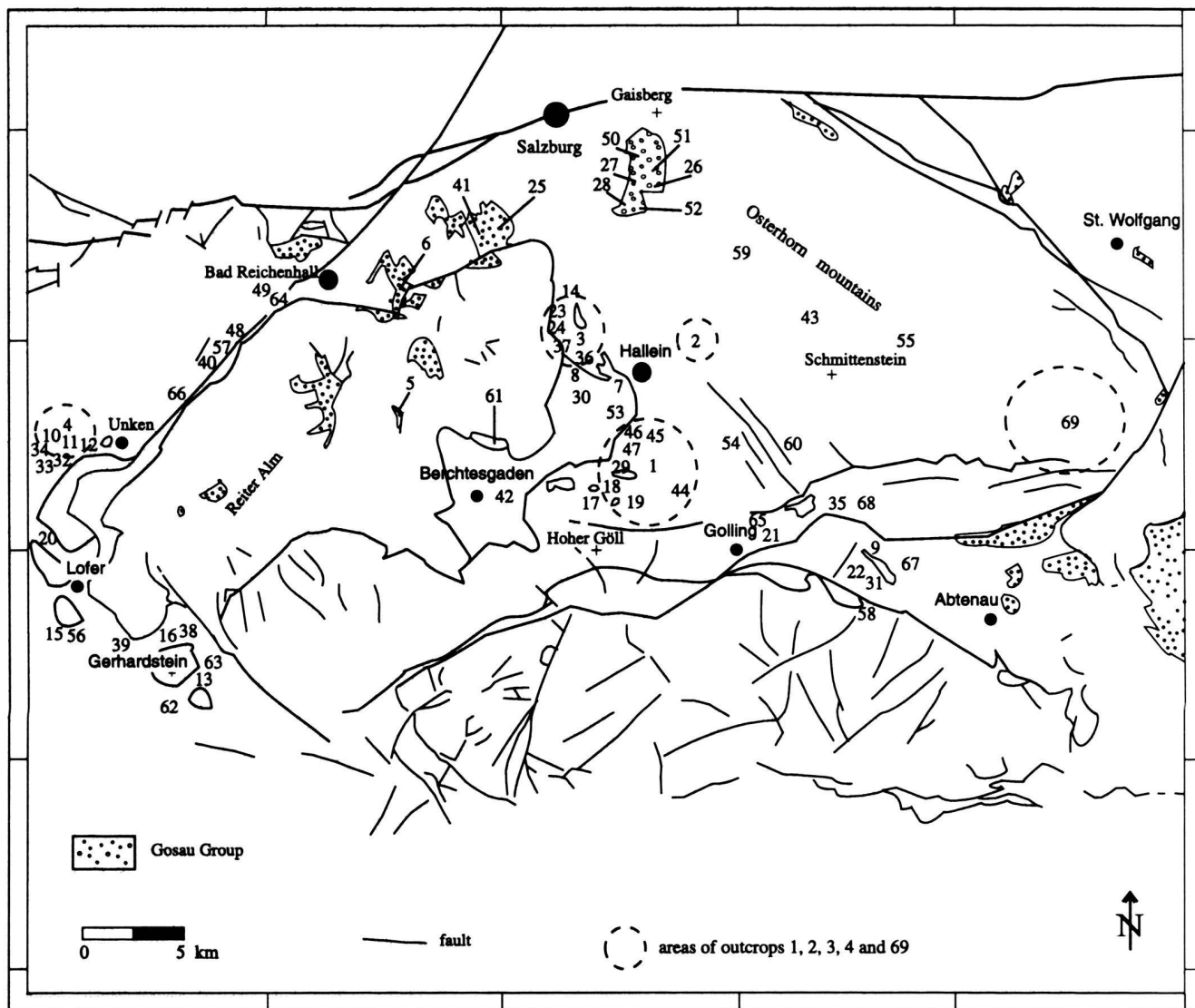
Fig. 12. Localities of the outcrops with data presented in Table 1 and 2.
