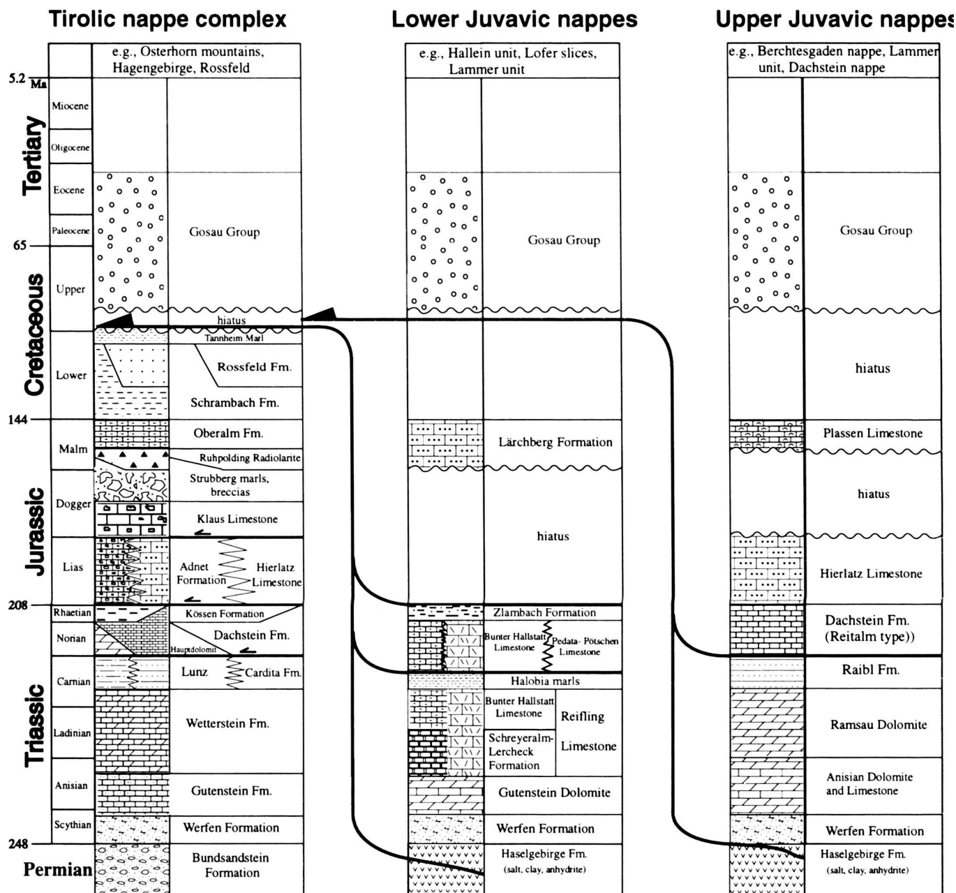
Fig. 3. Stratigraphy of the main tectonic elements of the central NCA with major decollement horizons.
