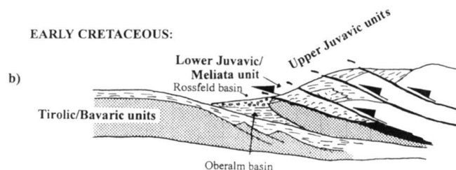
Fig. 5. Geological model for the possible paleogeographic origin of various nappe complexes within the central NCA during (a) Middle Triassic rifting and (b) or the emplacement of Juvavic nappes onto the Tirolitic unit during early Cretaceous, causing flexural bending of the Tirolitic units by thrust loading.
