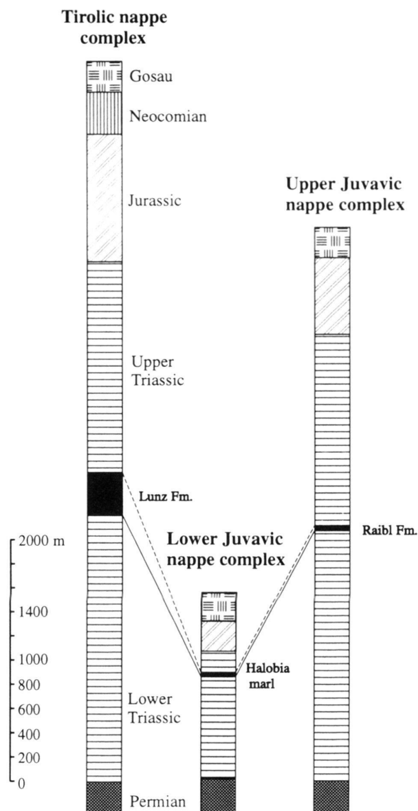
Fig. 4. Comparison of cumulative thickness within the main tectonic elements of the central NCA. Data from Plöschinger (1980).
