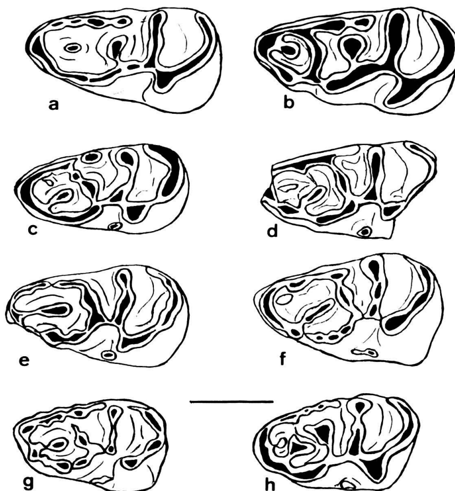
Fig. 2. D 4 of Issiodoromyini from the studied localities to show their increasing length.
