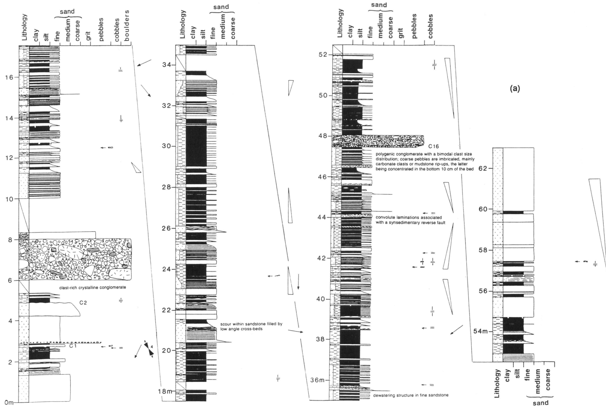
Plate 1. Measured section through the Sardona Quartzite Formation (lower part) at its type section at Jakobiweid (742.1/193.1; 1740 m) on Alp Sardona in Calfeisental.
