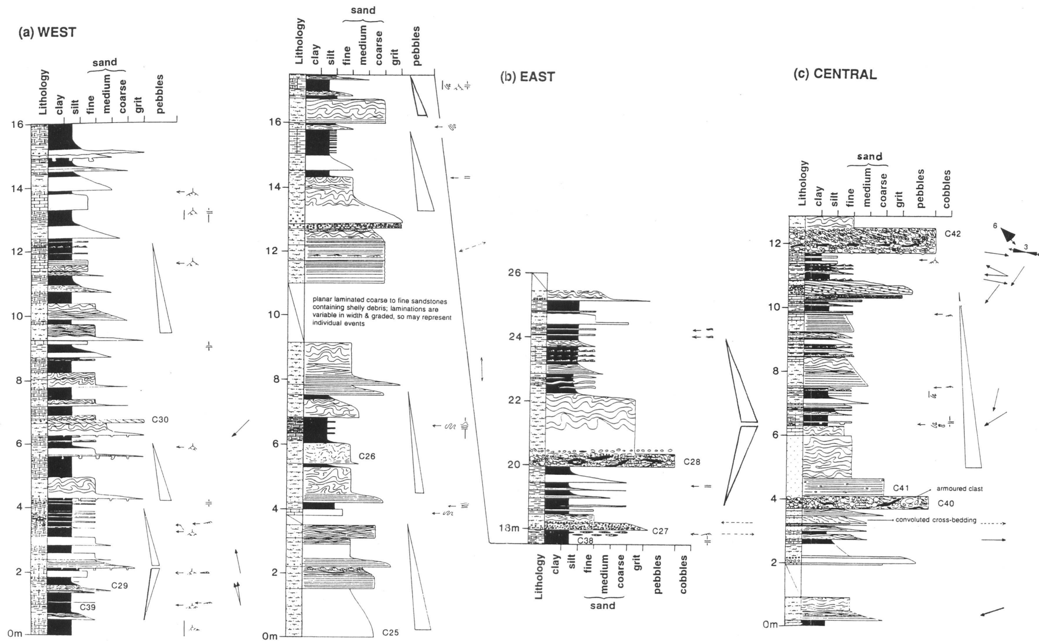
Plate 3. Measured sections through the Supraquartzite Flysch Formation at its type section at Plattenkopf, Alp Sardona, Calfeisentäl: (a) western section (741.4/199.8; 2260 m), (b) eastern section (741.9/199.8; 2200 m) and (c) central section (741.8/199.8; 2240 m).
