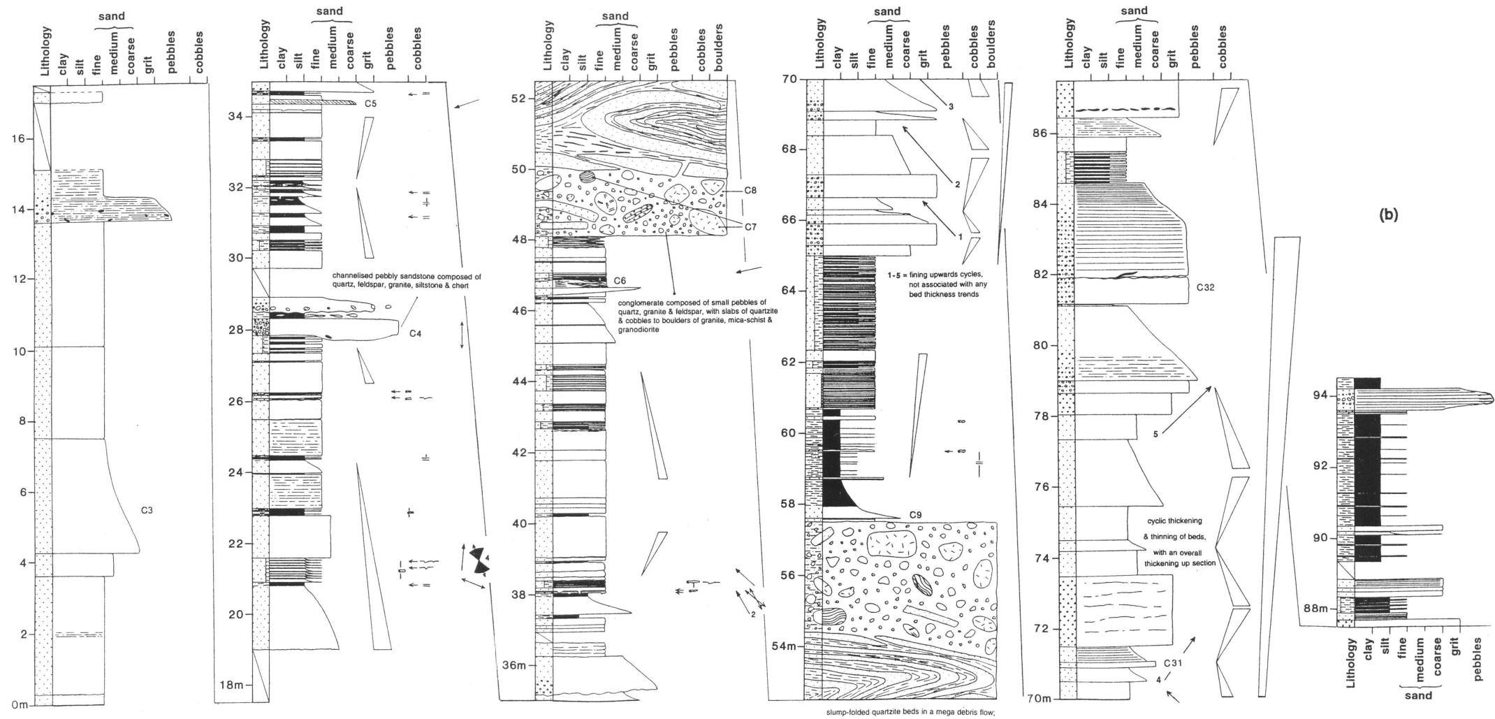
Plate 2. Measured section through the Sardona Quartzite Formation (upper part) at its type section at Trosegg Tobel (741.1/198.0; 1800 m) on Alp Sardona in Calfeisental.
