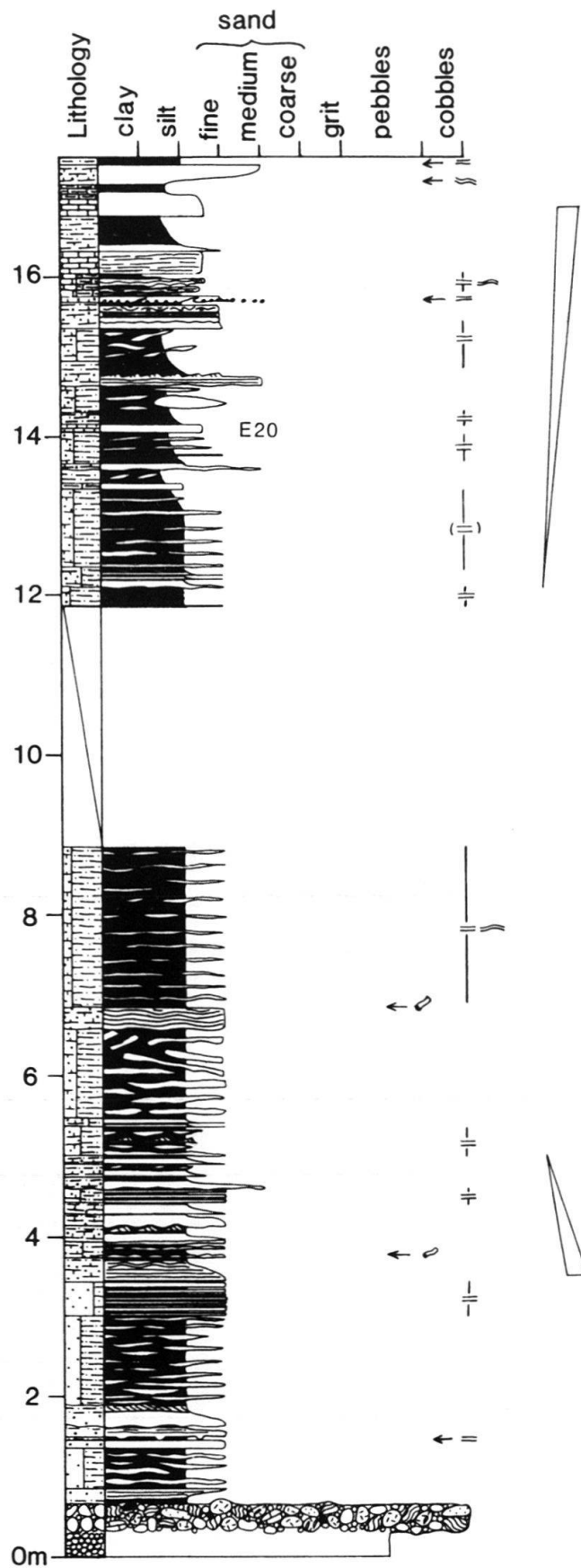
Fig. 5. Measured section through the 'Rindermättli Formation' of Wegmann (1961), which forms the basal part of the Infraquartzite Flysch Formation in the Elm district (733.3/195.4; 1750 m).
