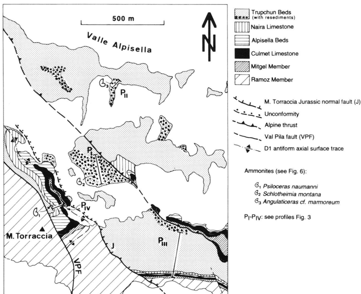
Fig. 7. Geological map of the M. Torraccia area.
