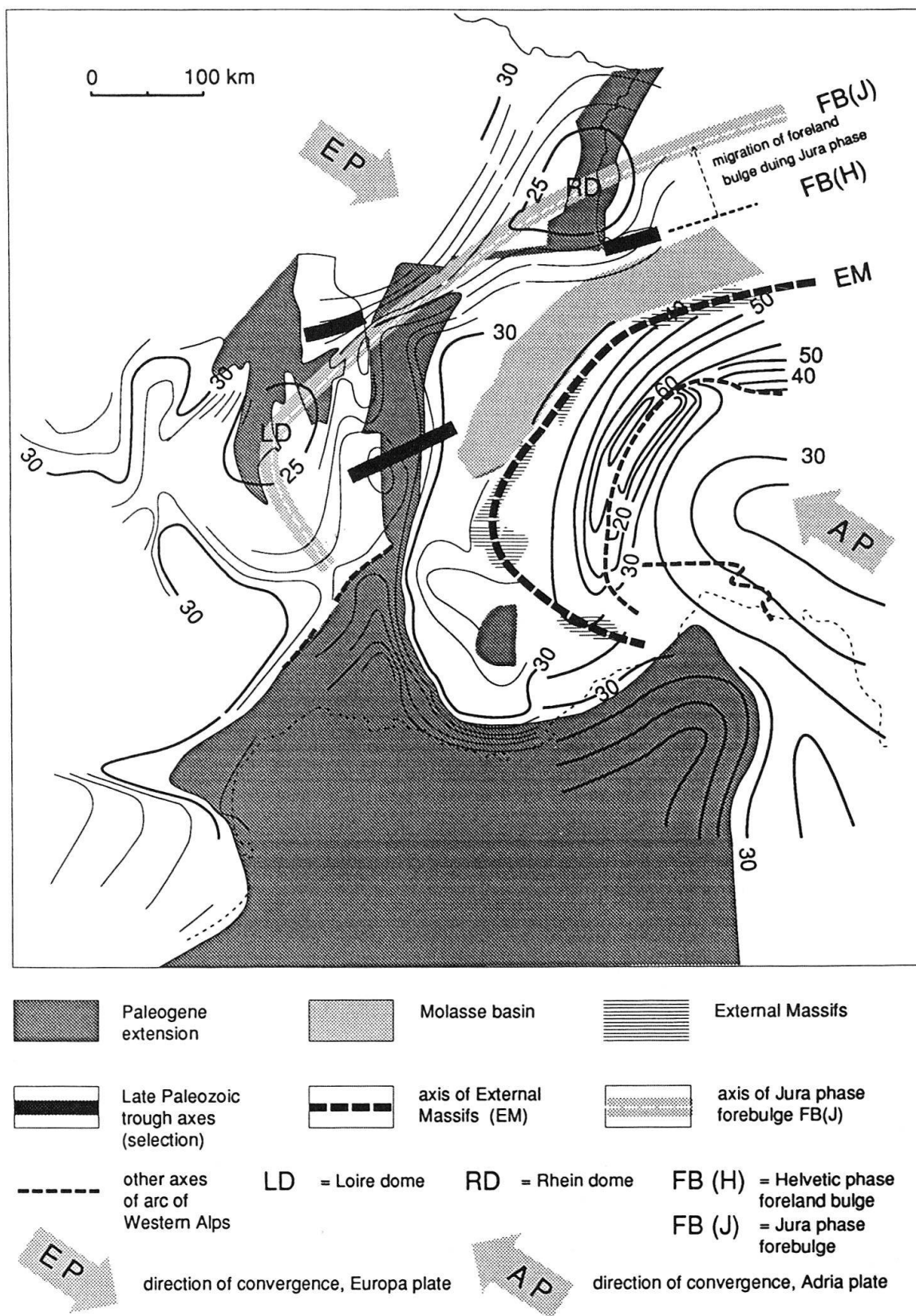
Fig. 14. The estimated positions of the foreland bulges attributable to the Helvetic-Insubric phase (FBH) and the Jura phase (FBJ), superimposed on the isobaths of the Moho (after Hirn 1980, Giese). Very dark bands: examples of known late Paleozoic troughs. Dark shading: Paleogene to Early Miocene extensional structures.
