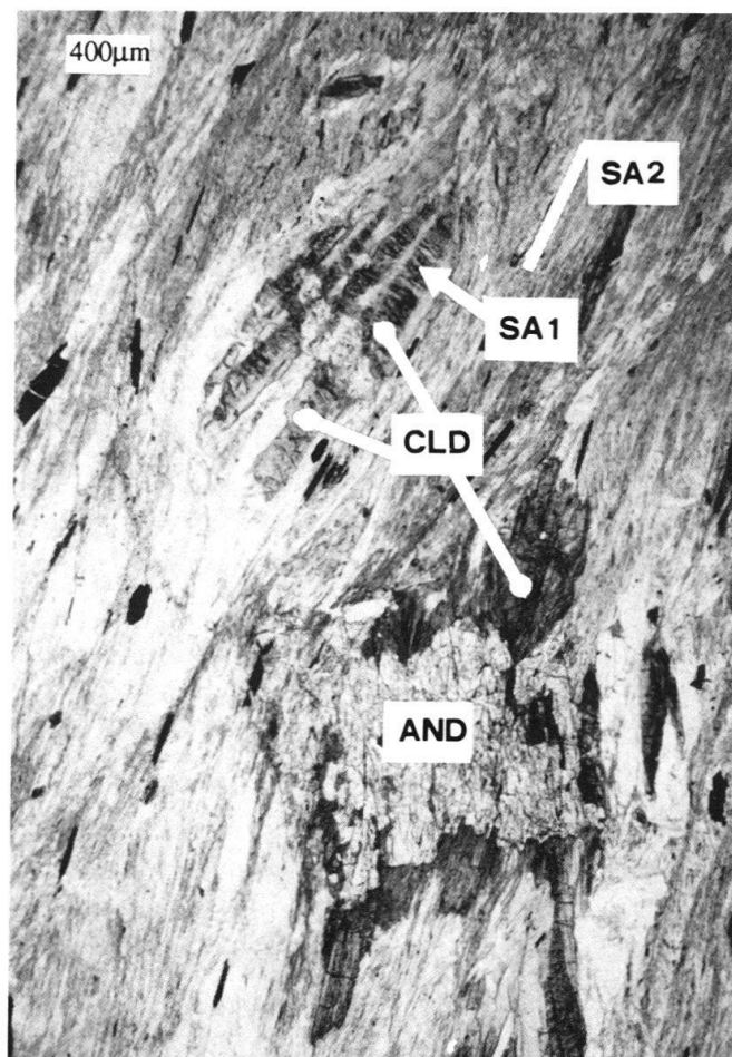
Fig. 5c (top): SX bearing garnet, SE biotite (BIO), SA1 and SA2. Polarized light. d (bottom): Post-SA1/pre-SA2 chloritoid (CLD) and post-tectonic andalusite (AND). Polarized light.
