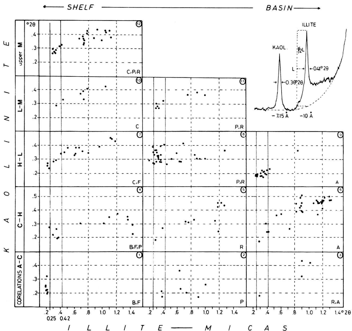
Fig. 15. Platform to basin variation in the crystallinity index, measured at half the elevation of peaks, (001) of illite at about 10 Å, and (002) of kaolinite at 7.15 Å. The correlation fields, numbered from 1 to 12, are arranged in vertically successive blocks, which are related to the stratigraphic correlations A to M in the left column (cf. Fig. 9). Letters down right in individual cases are abbreviated names of sampled sections: B for Bressaucourt, C for Courgenay, etc.
