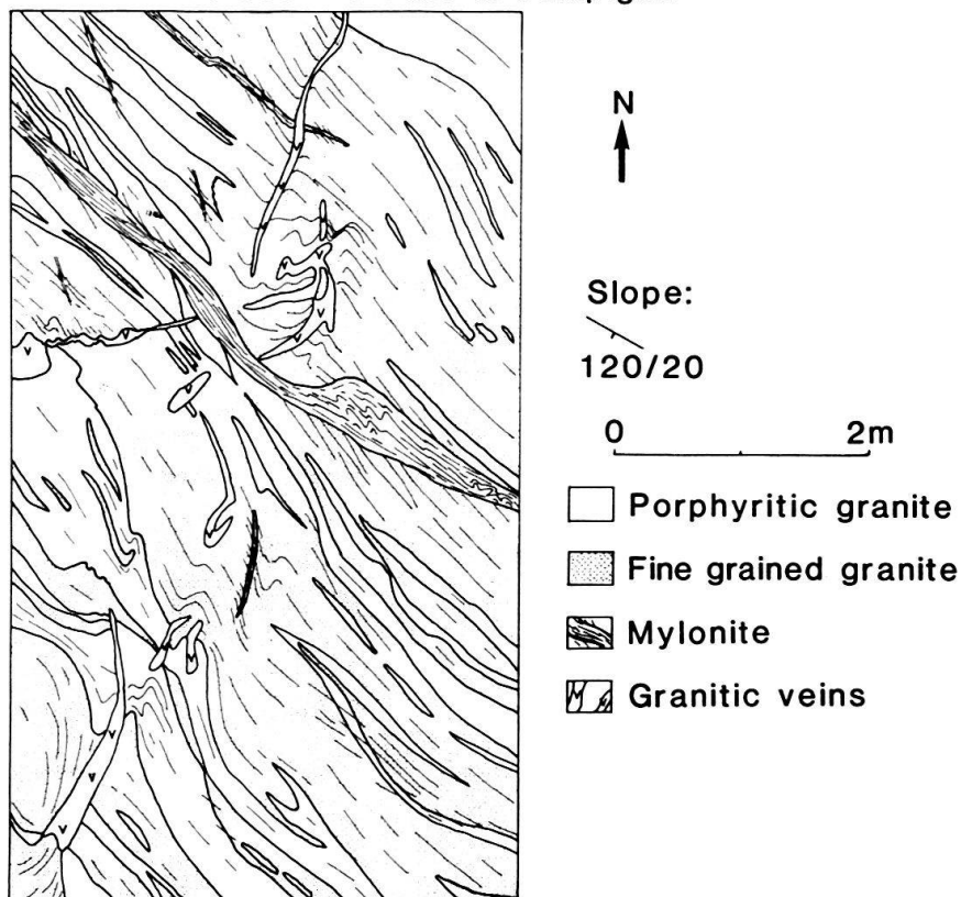
Fig. 8. Detailed geological map of highly deformed basement, including shear zone, in the Campiglia Valley. Grid reference refers to grid of Figure 5. The features shown in this figure represent highly deformed versions of the lithologies illustrated in Figure 7. The xenoliths are flattened subparallel to the main (D2) fabric and the outcrop cut by a shear zone within which are developed mylonites and non-cylindrical folds of the mylonitic fabric.
