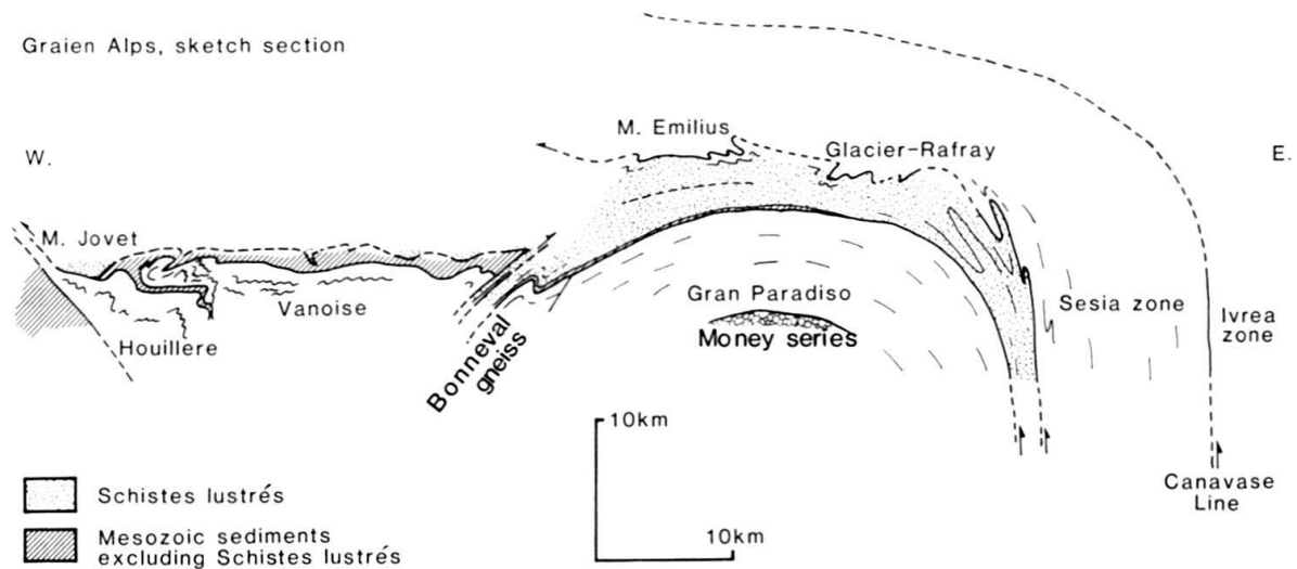
Fig. 3. An E-W geological cross section (scale approximate) through part of the Western Alps with some extrapolation along strike. Drawn after the authors own observations, ELLENBERGER (1958) for the Vanoise, and NERVO & POLINO (1976) for the Monte Emilius and Glacier-Rafay klippen.
