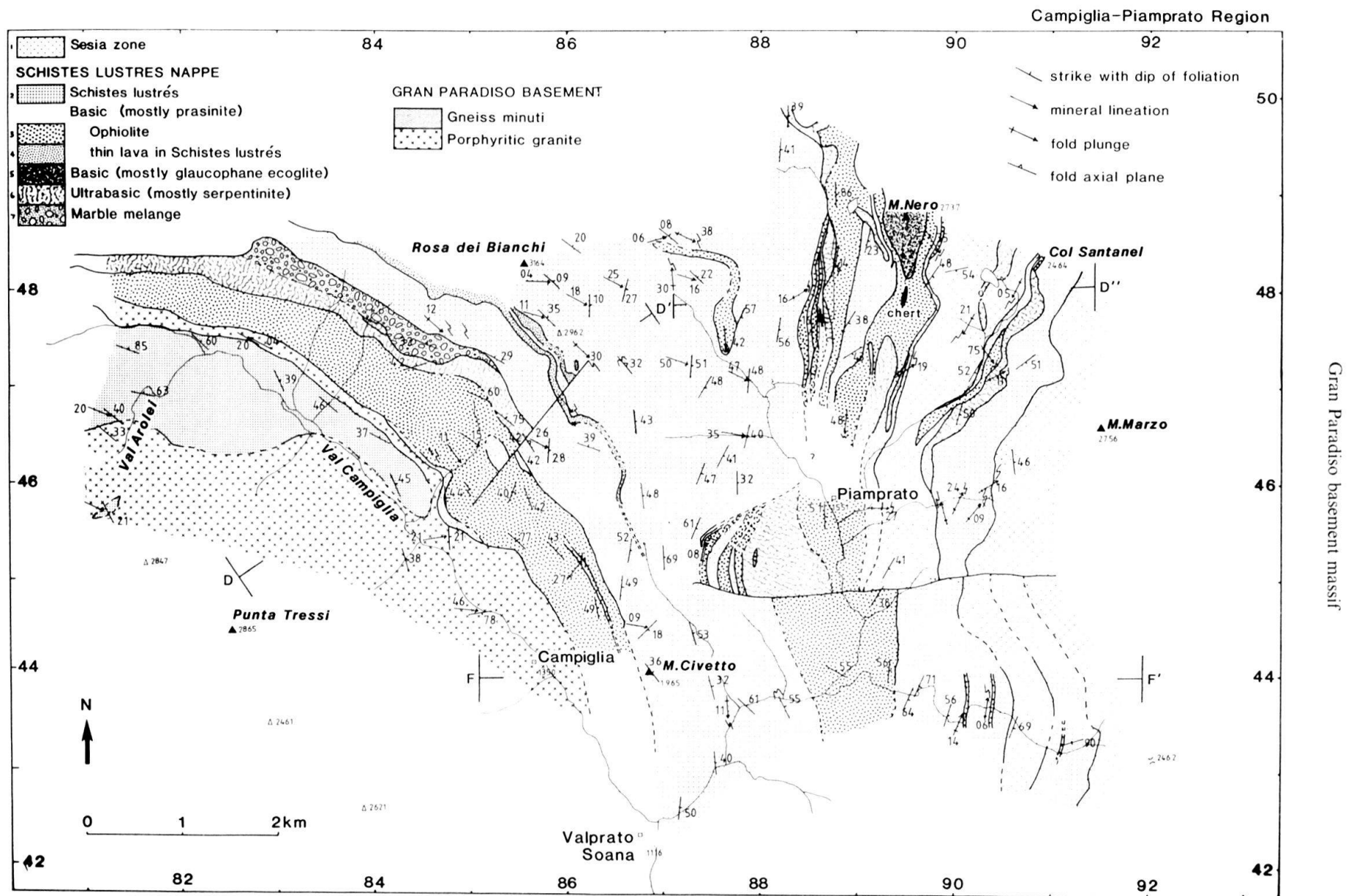
Fig. 5. Geological map of the northeastern Gran Paradiso. Map based on mapping at 1:25,000 by the author. This map is complementary to the sections DD'D'' and FF' in Figure 4. Grid references are taken from the Valprato Soana, Carta D'Italia, 1:25,000, sheet 42, IV, S.O.
