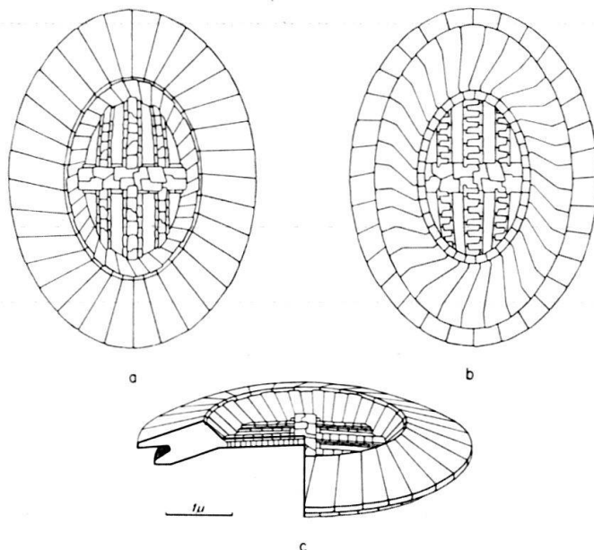
Fig. 28. Schematic drawings of Sollasites horticus (STRADNER, ADAMIKE & MARESCH, 1966) BLACK, 1968, with straight and slightly curved outer bars.
