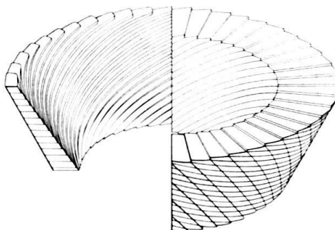
Fig. 29. Schematic drawing of the wall construction of the family Zygolithaceae NOËL, 1965, ex BLACK, 1968, emend. GRÜN.
