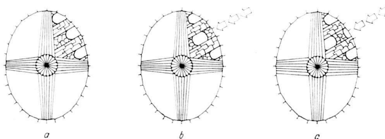
Fig. 19. Schematic drawings of the central area.
