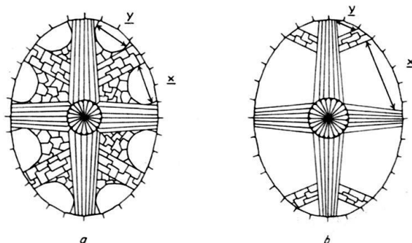
Fig. 18. Schematic drawings of Retecapsa crenulata (BRAMLETTE & MARTINI, 1964) GRÜN n. comb. a) distal view – b) proximal view.
