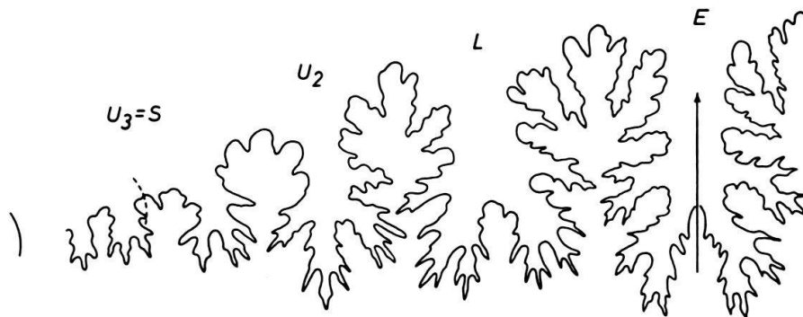
Fig. 7. External suture line of T. blaisoni COLLIGNON. Holotype, M. Collignon coll. No. 474. Lower Cenomanian, Beraketa-Sakondry (Madagascar). At WH 10 mm. Ca. 5/1.
