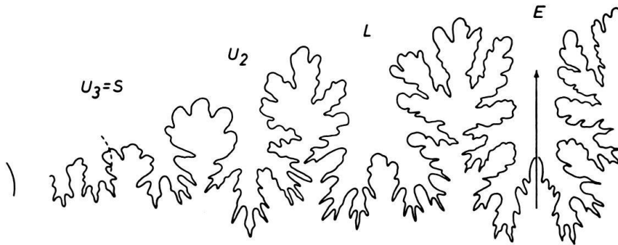
Fig. 7. External suture line of T. blaisoni COLLIGNON. Holotype, M. Collignon coll. No. 474. Lower Cenomanian, Beraketa-Sakondry (Madagascar). At WH 10 mm. Ca. 5/1.
