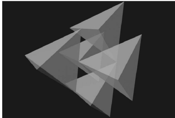
Fig. 5 Touching tetrahedrons
