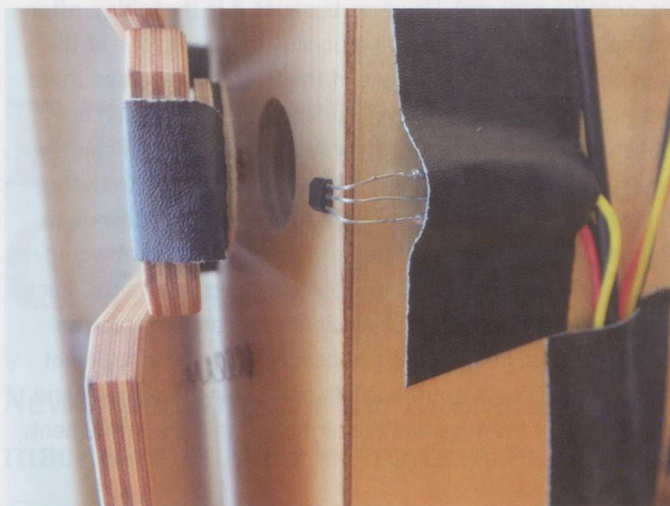
Figure 1: This picture shows a magnet which is under the tape on the key, and the magnetic field sensor on the instrument's body. © Simone Conforti
