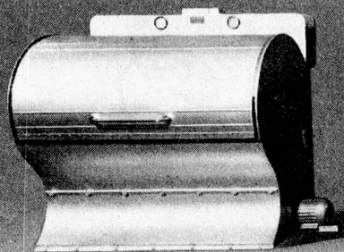
Type III
