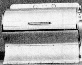
Type II
