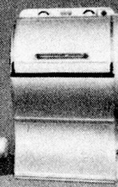
Type Ia
