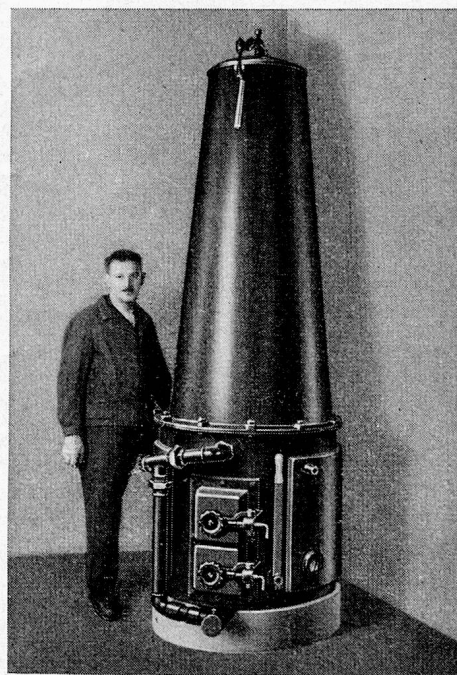
Holzgas-Generator
