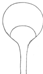
Fig. 41. Rhizopus nigricans .
