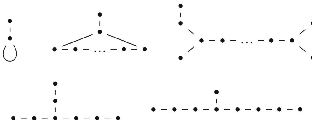
Figure 1. The wild graphs \widetilde{A}_0, \widetilde{A}_n (minimal for 1 \leq n \leq 6 ), \widetilde{D}_n (minimal for 4 \leq n \leq 8 ), \widetilde{E}_6 and \widetilde{E}_7 . If one of these graphs has the index j \geq 0 in the name, it has j + 2 vertices.
