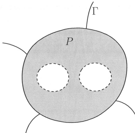
Figure 3. In this example the dashed lines are removed from \Gamma .
