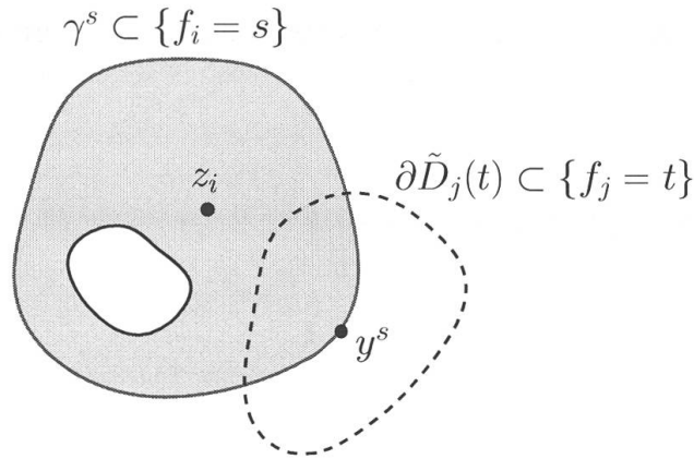
Figure 2. An example for the setting described in the proof of Theorem 1.7. In this example, the gray region is V_i(s) , the solid lines are the s -level set of f_i , and the outer component is \gamma^s . The dashed line is the boundary of \tilde{D}_j(t) , which is a part of the t -level set of f_j , for some t < f_j(y^s) .
