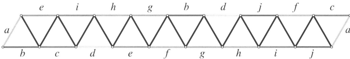
Figure 6. Genus 5 example that saturates bound in Proposition 3.1.
