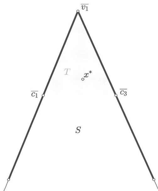
Figure 12. The point x^* in the triangle T .
