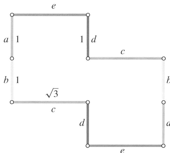
Figure 1. A pair (X, \omega) that has ten systoles: By identifying parallel sides with the same letters, we obtain a Riemann surface X . The one form dz in the plane defines a holomorphic 1-form on X .
