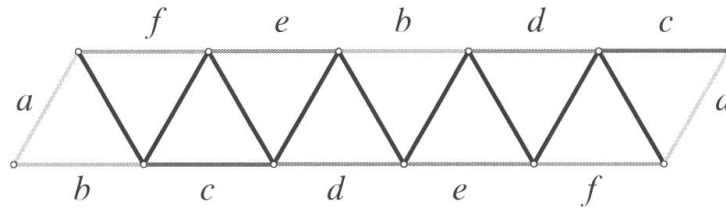
Figure 4. Genus 3 example that saturates bound in Proposition 3.1. Glue the edges of the polygon according to the labels. Each edge is a systole, the 1-form \omega has exactly one zero, and no two Delaunay edges are homotopic.
