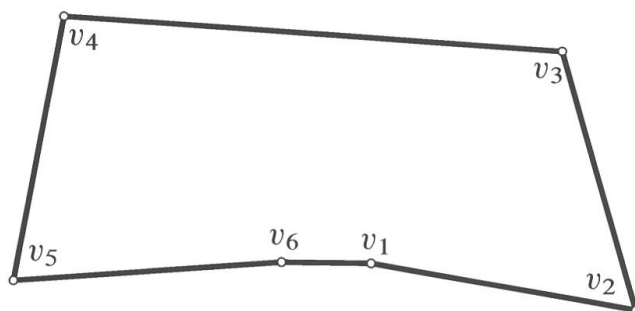
Figure 18. The points v_i, i = 1, \dots, 6 .
