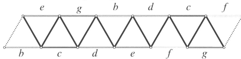
Figure 7. Glue solid edges of the polygon that have the same label to obtain the Delaunay triangulation associated a holomorphic 1-form on a surface of genus two having two boundary components.
