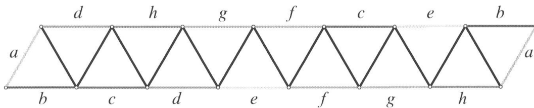
Figure 5. Genus 4 example that saturates bound in Proposition 3.1.
