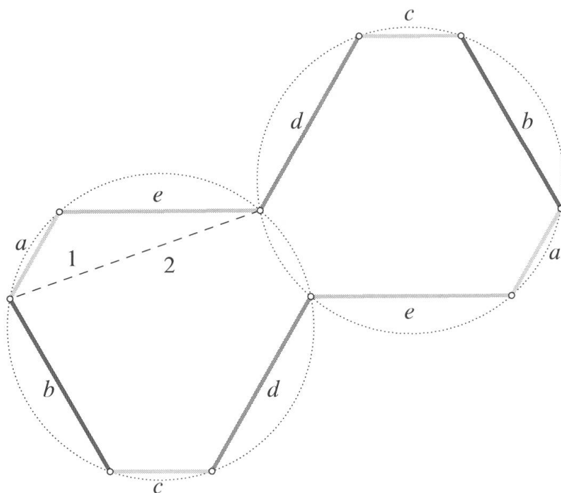
Figure 2. A surface (X, d_{\omega}) whose systolic ratio equals the constant in (1.1). The surface is obtained from gluing parallel sides of two isometric cyclic hexagons in \mathbb{C} . Each hexagon has a rotational symmetry of order 3. The 1-form \omega corresponds to dz in the plane.
