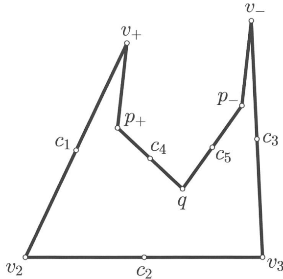
Figure 13. The polygon P .
