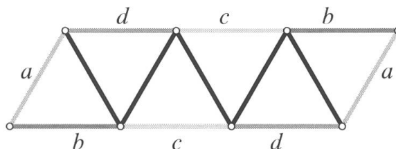
Figure 3. The genus two surface (X, d_\omega) that achieves the optimal bounds in \mathcal{H}(2) .
