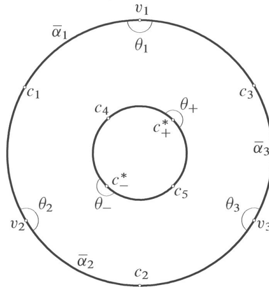
Figure 11. The topological annulus K .
