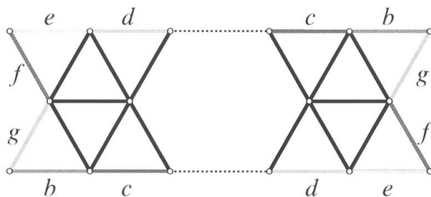
Figure 8. Glue edges of the polygon that have the same label to obtain the Delaunay triangulation associated to a holomorphic 1-form on a surface of genus g . The surface is hyperelliptic, the 1-form \omega has exactly one zero, and there are exactly 6g - 5 homotopy classes of systoles.
